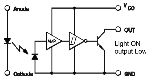
OPB917IO CZ Inverted Open-Collector
