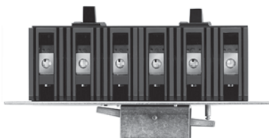
Walking Beam Mechanical Interlock Requires 2 circuit breakers with WB suffix, 1 walking beam assembly and 1 mounting pan.
