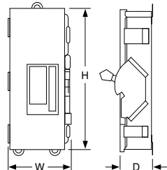
Enclosures for IK250DS and IK250AWK
