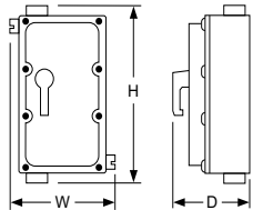
Enclosures for IK250DS and IK250AWK
