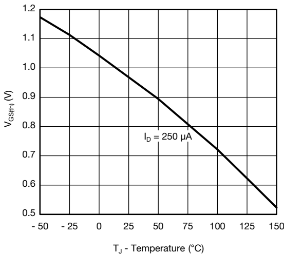
Threshold Voltage
