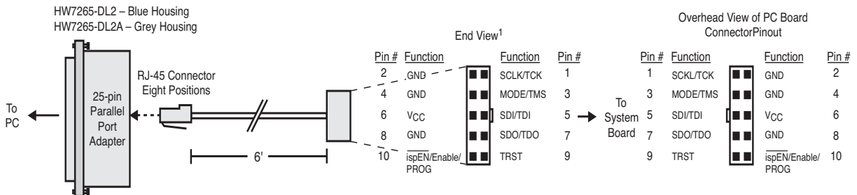
Figure 6. Programming Cable In-System Programming Interface for the PC (HW7265-DL2 or HW7265-DL2A)
