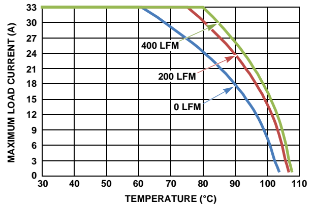
FIGURE 16. 12V_{\text{IN}} TO 1V_{\text{OUT}}
