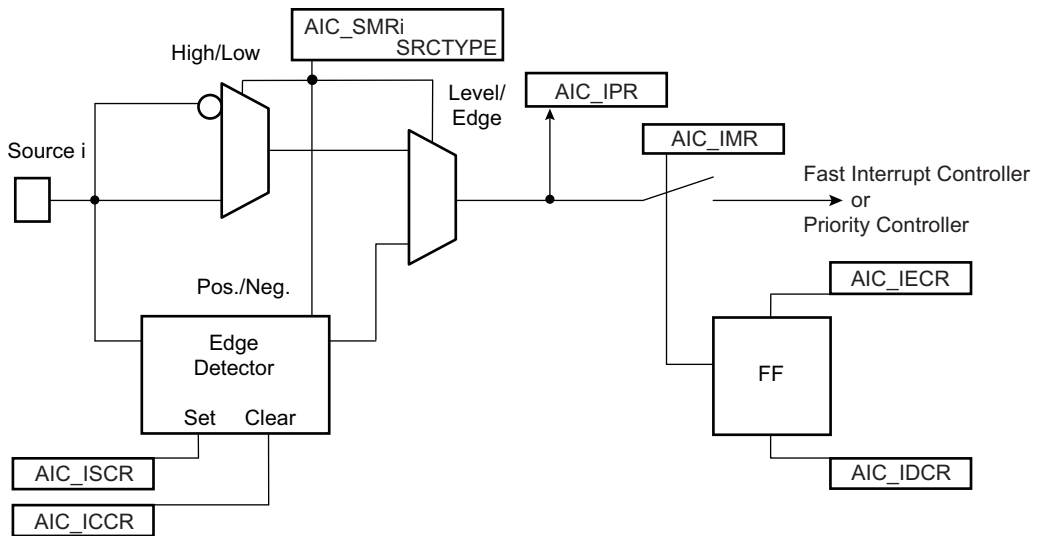
Figure 18-5. External Interrupt Source Input Stage
