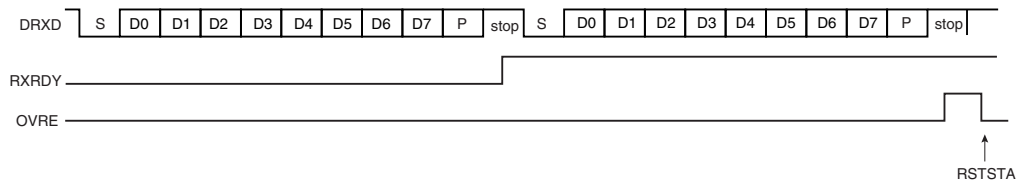
Figure 42-7. Receiver Overrun
