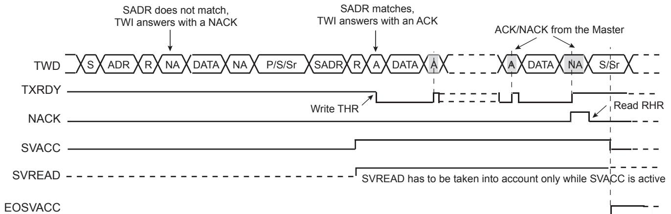
Figure 40-25. Read Access Ordered by a MASTER
