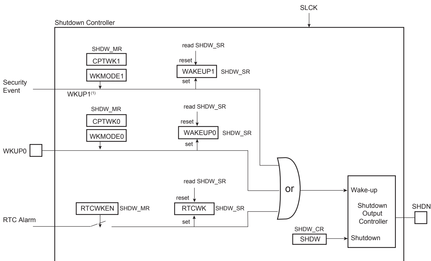
Figure 21-1. Shutdown Controller Block Diagram
