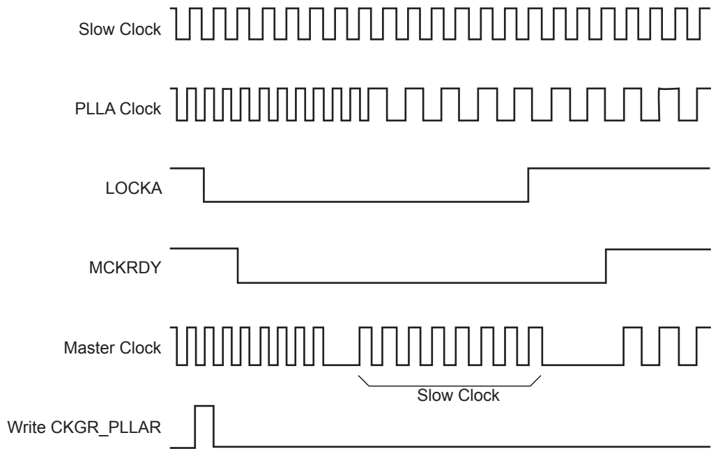
Figure 27-7. Change PLLA Programming
