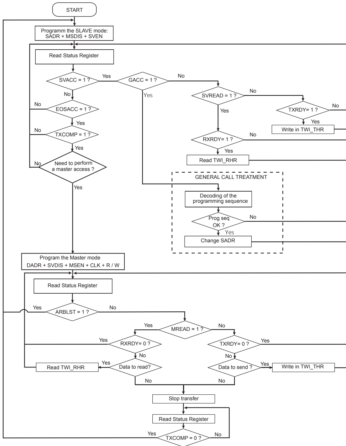
Figure 40-23. Multi-master Flowchart
