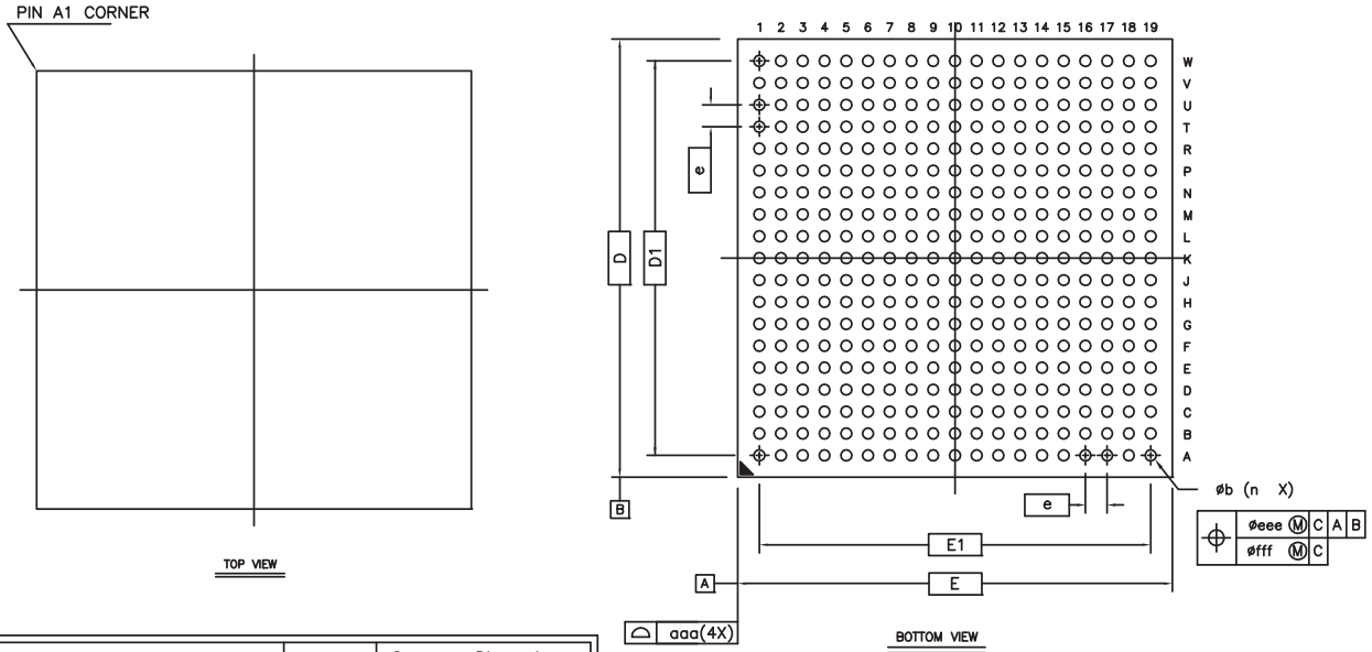
Figure 57-1. 361-ball LFBGA Package Drawing
