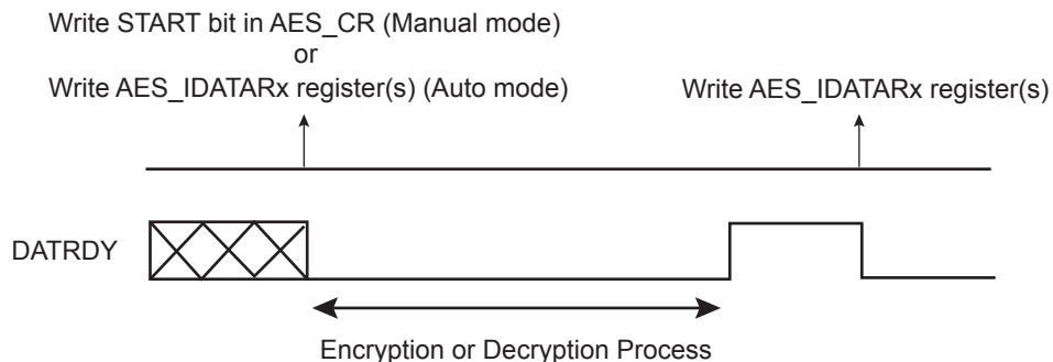
Figure 50-2. Manual and Auto Modes with AES_MR.LOD = 1
