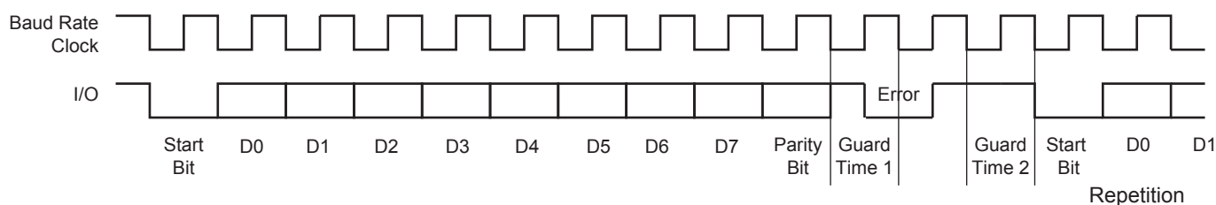
Figure 44-30. T = 0 Protocol with Parity Error
