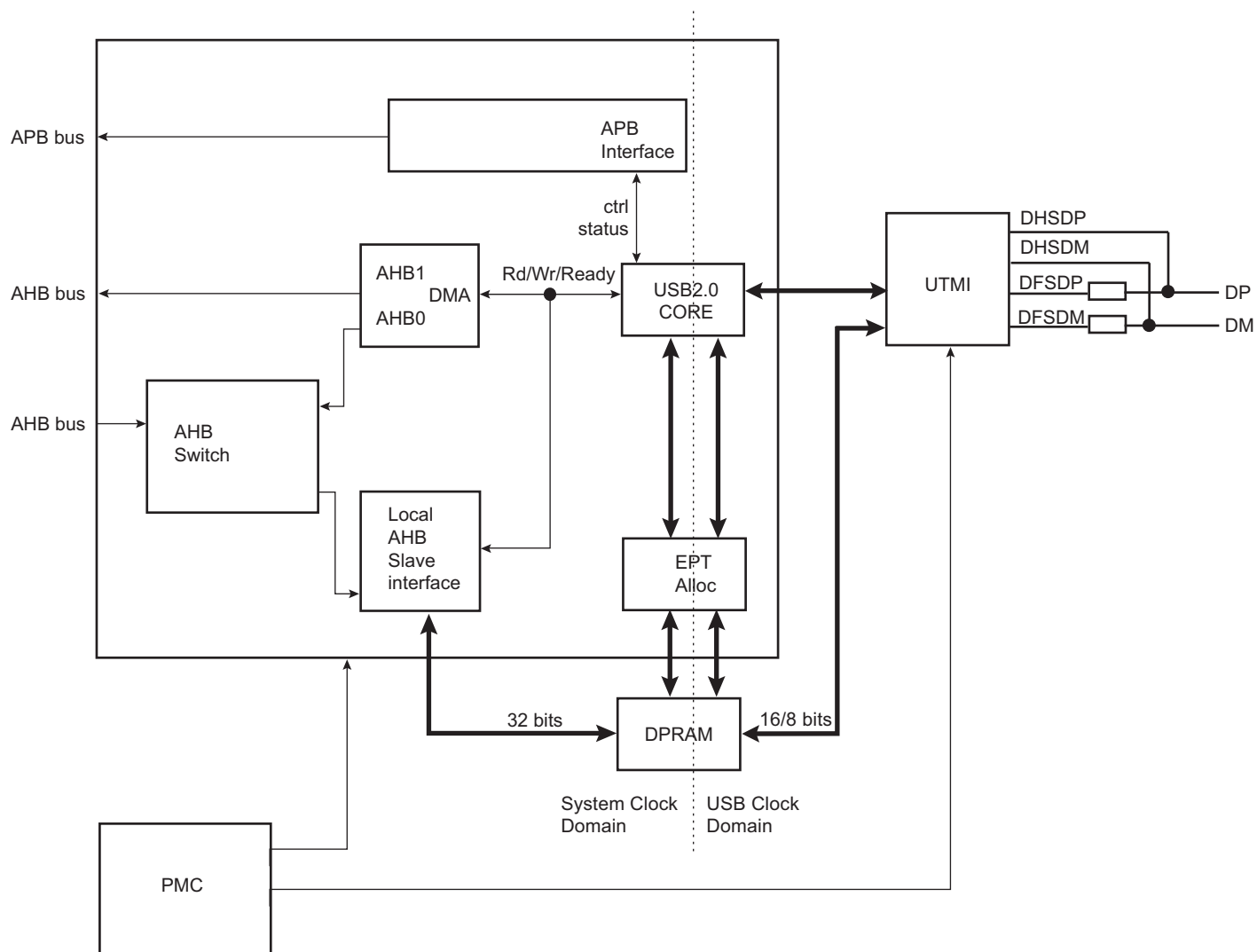
Figure 35-1. Block Diagram
