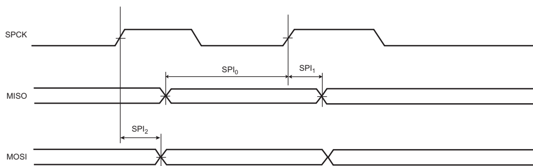
Figure 56-8. SPI Master Mode 1 and 2
