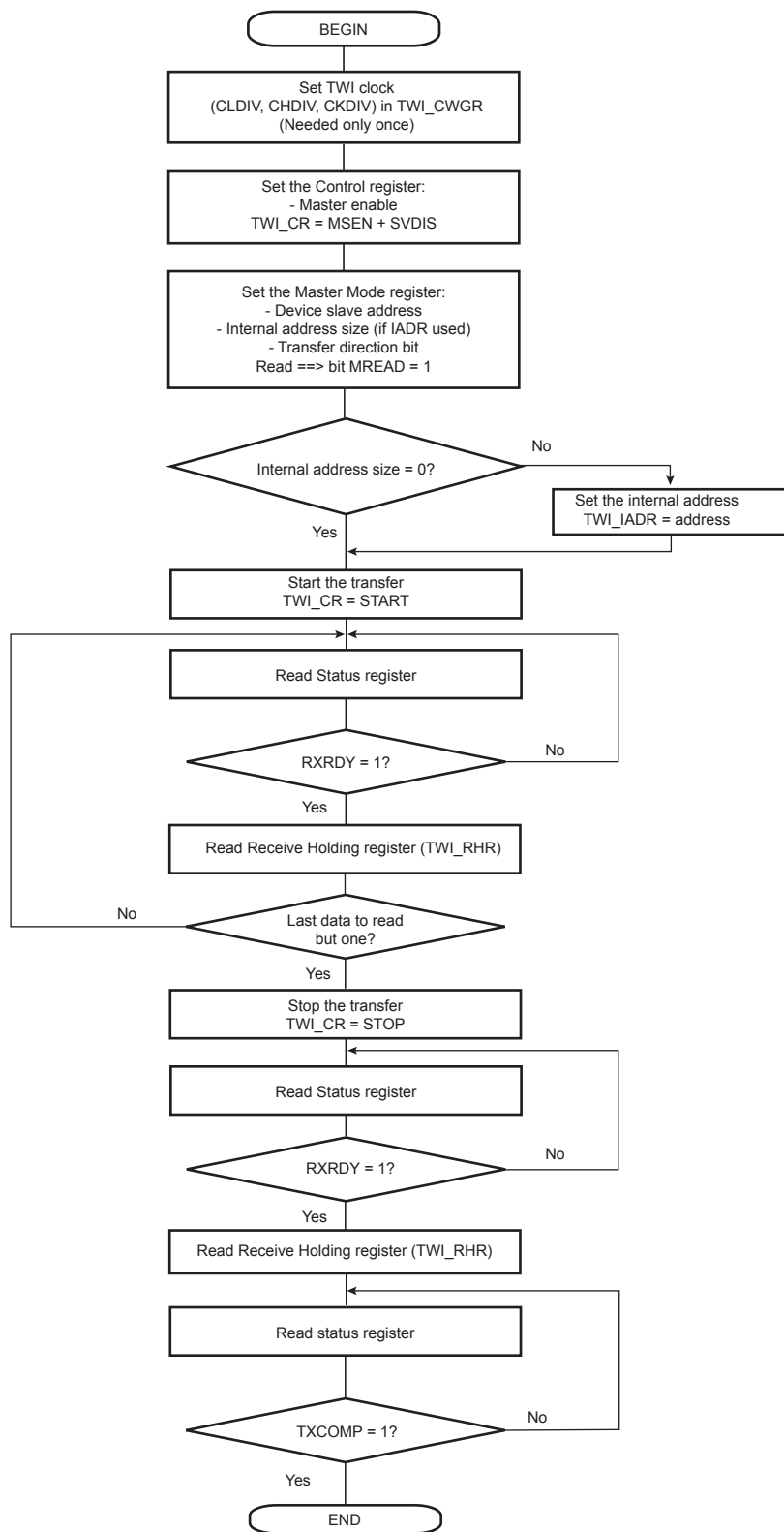
Figure 40-20. TWI Read Operation with Multiple Data Bytes with or without Internal Address
