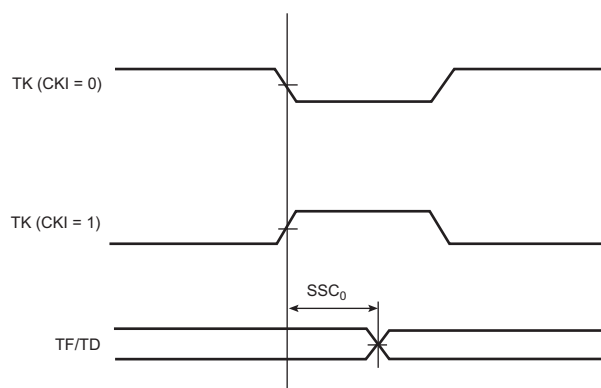
Figure 56-15. SSC Transmitter, TK and TF in Output
