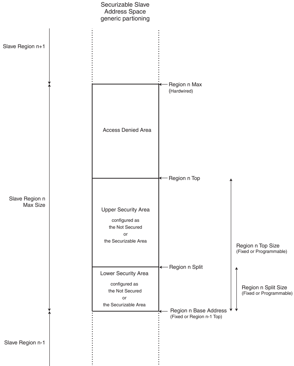
Figure 16-1. Generic Partitioning of the AHB Slave Address Space
