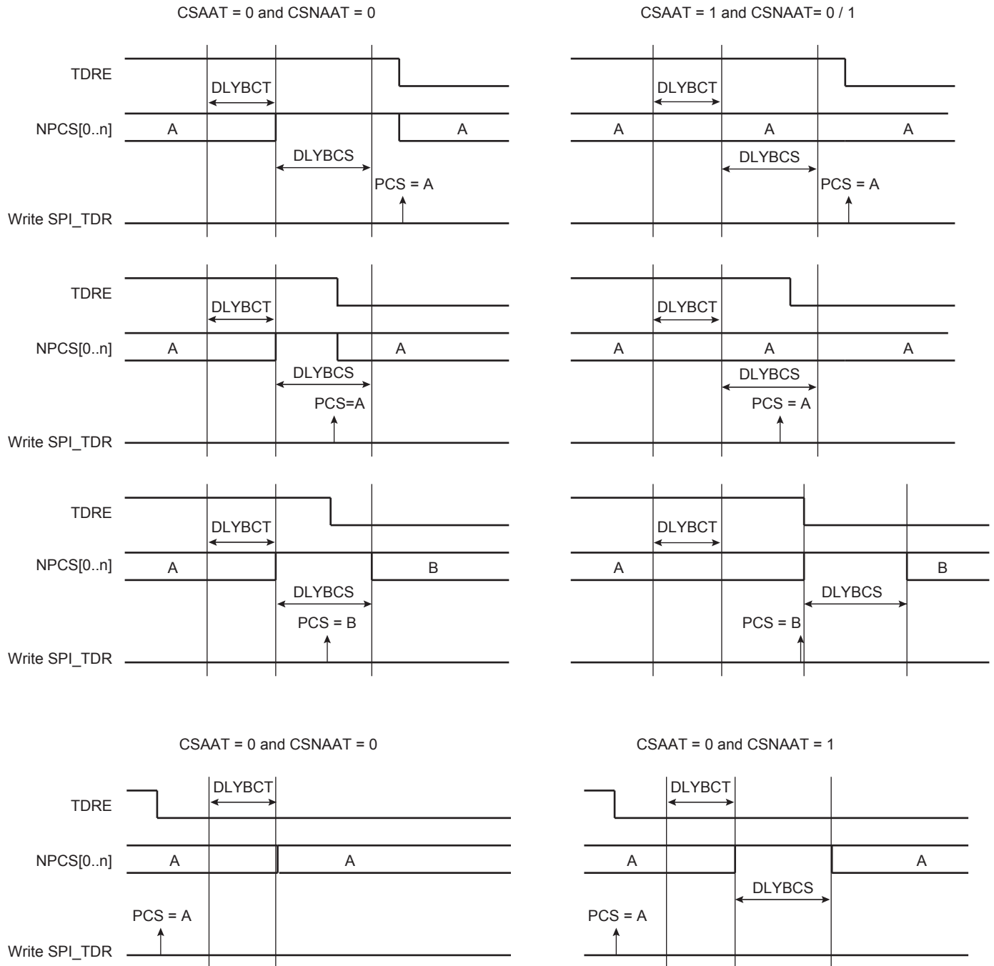
Figure 39-10. Peripheral Deselection
