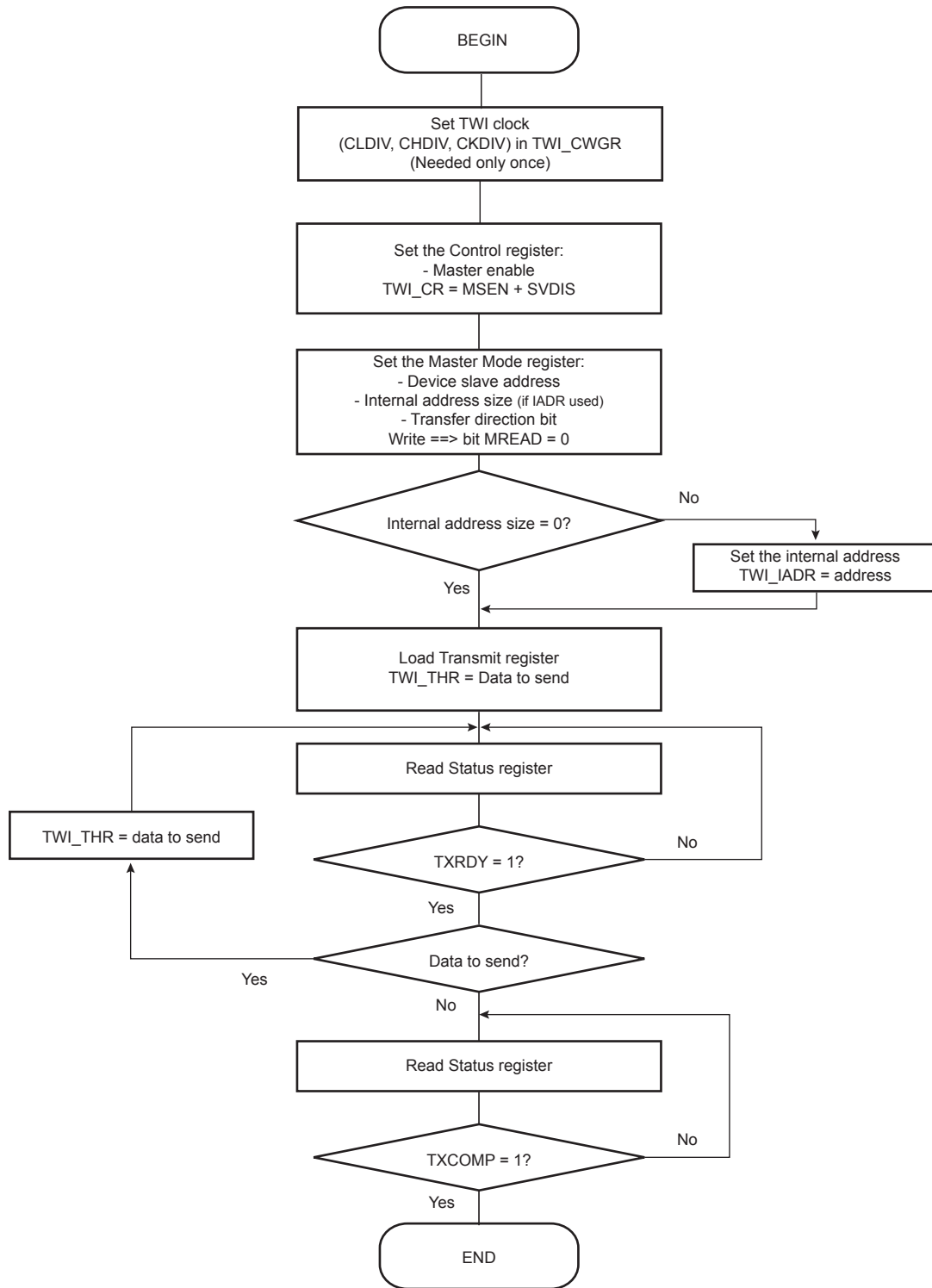
Figure 40-17. TWI Write Operation with Multiple Data Bytes with or without Internal Address
