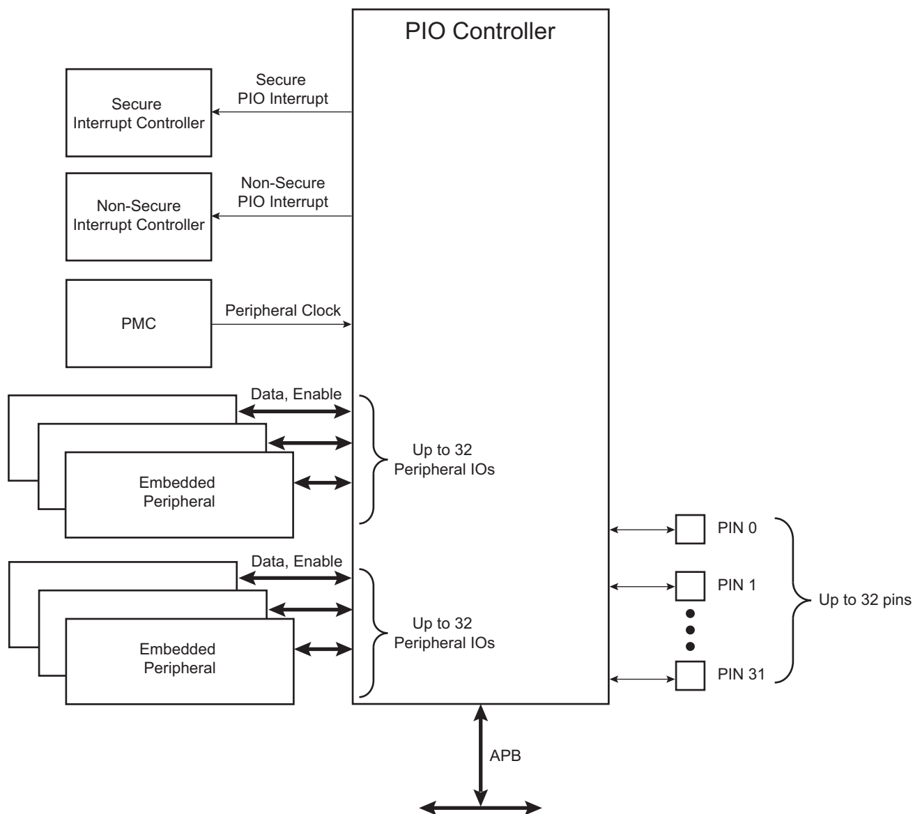
Figure 28-1. Block Diagram
