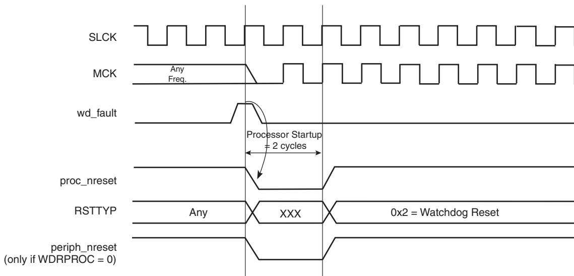
Figure 20-7. Watchdog Reset
