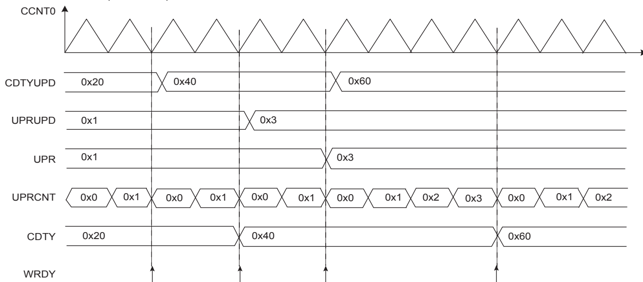
Figure 47-12. Method 2 (UPDM = 1)
