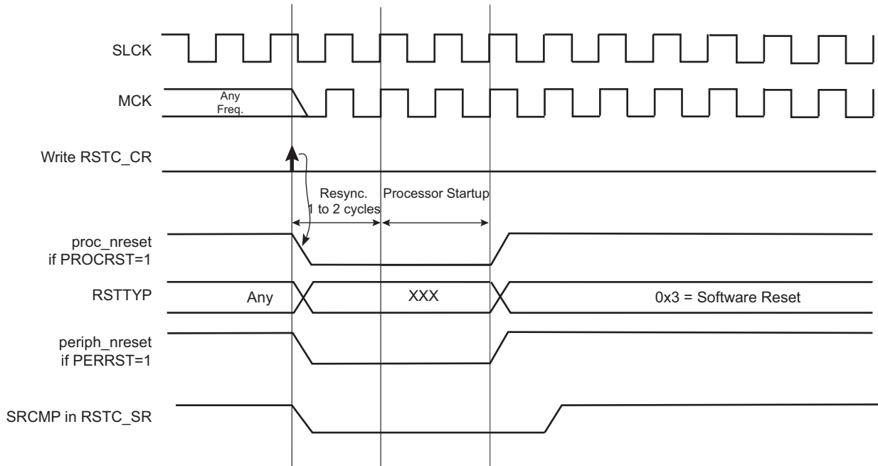
Figure 20-6. Software Reset
