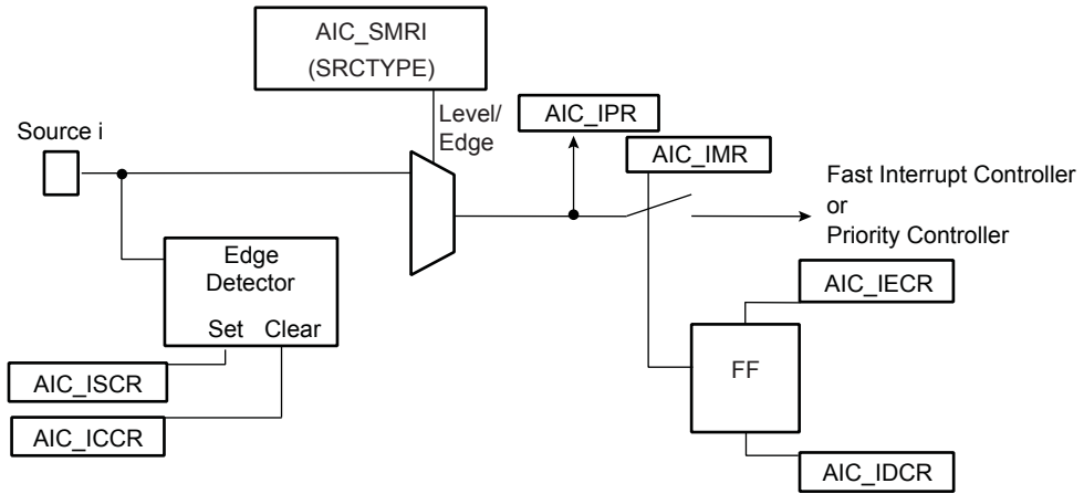
Figure 18-4. Internal Interrupt Source Input Stage
