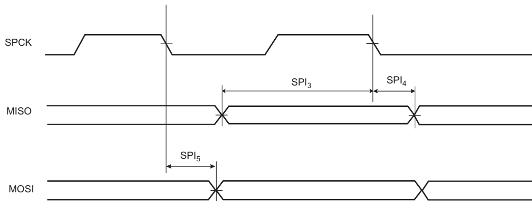
Figure 56-9. SPI Master Mode 0 and 3
