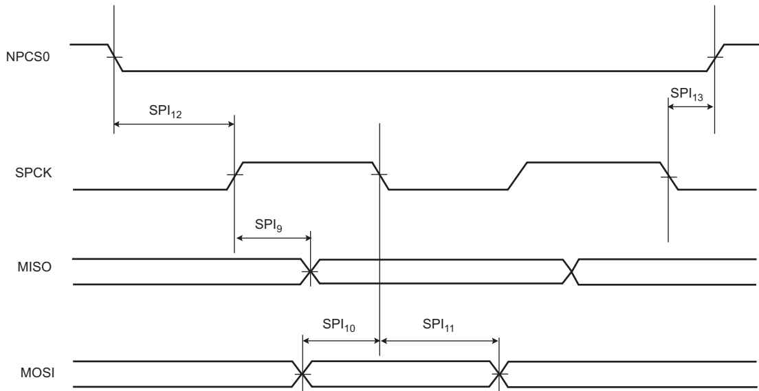
Figure 56-11. SPI Slave Mode 1 and 2
