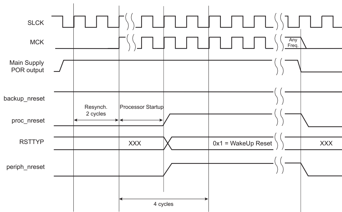
Figure 20-4. Wake-up Reset
