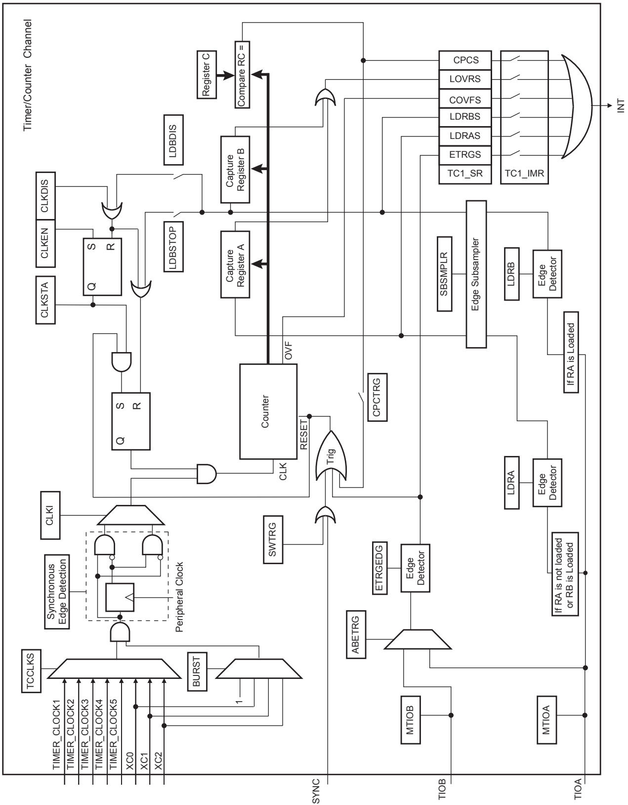
Figure 46-6. Capture Mode
