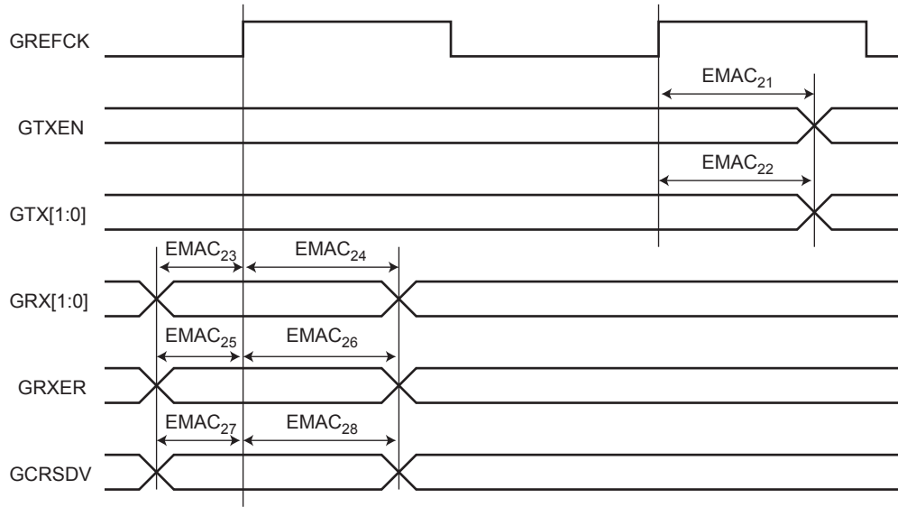
Figure 56-27. Ethernet MAC RMI Timings
