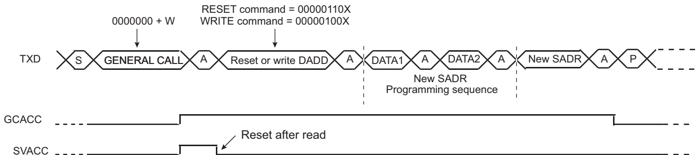
Figure 40-27. Master Performs a General Call
