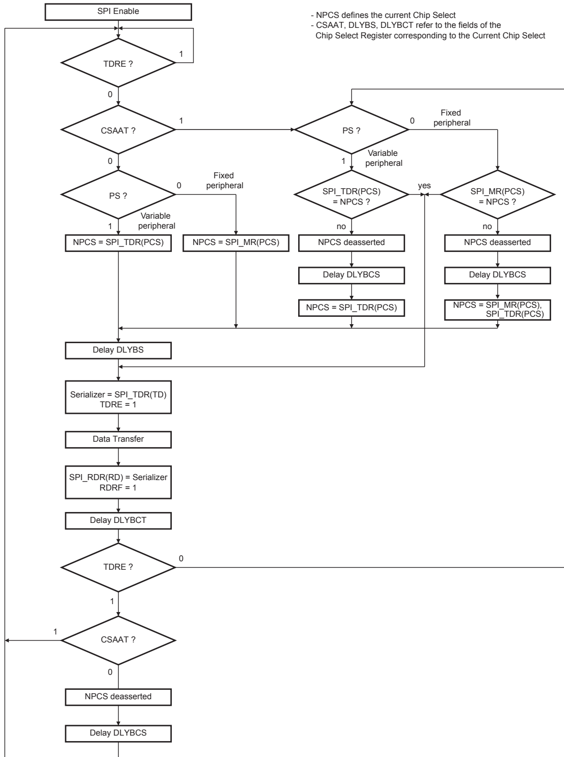
Figure 39-6. Master Mode Flow Diagram
