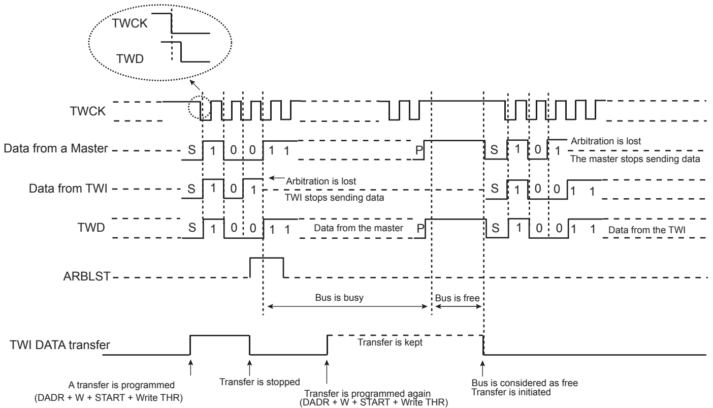
Figure 40-22. Arbitration Cases
