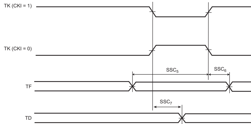
Figure 56-18. SSC Transmitter, TK and TF in Input
