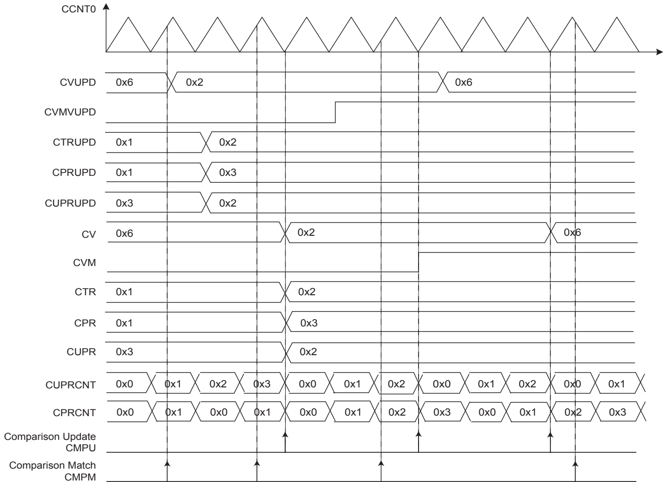
Figure 47-16. Comparison Waveform
