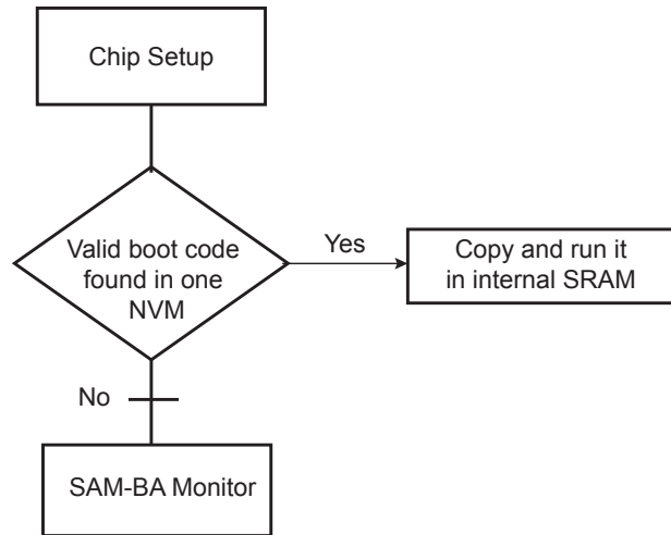
Figure 13-1. ROM Code Algorithm Flow Diagram
