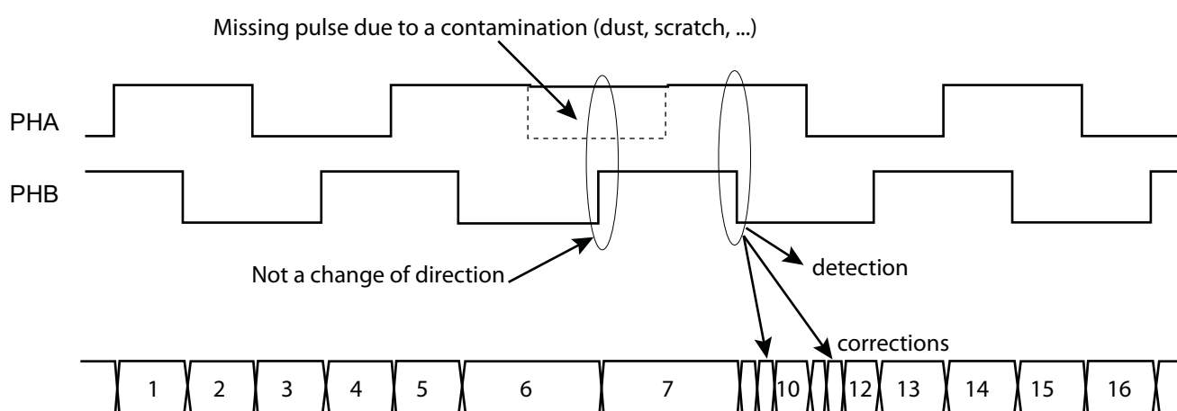
Figure 46-22. Detection and Auto-correction of Missing Pulses
