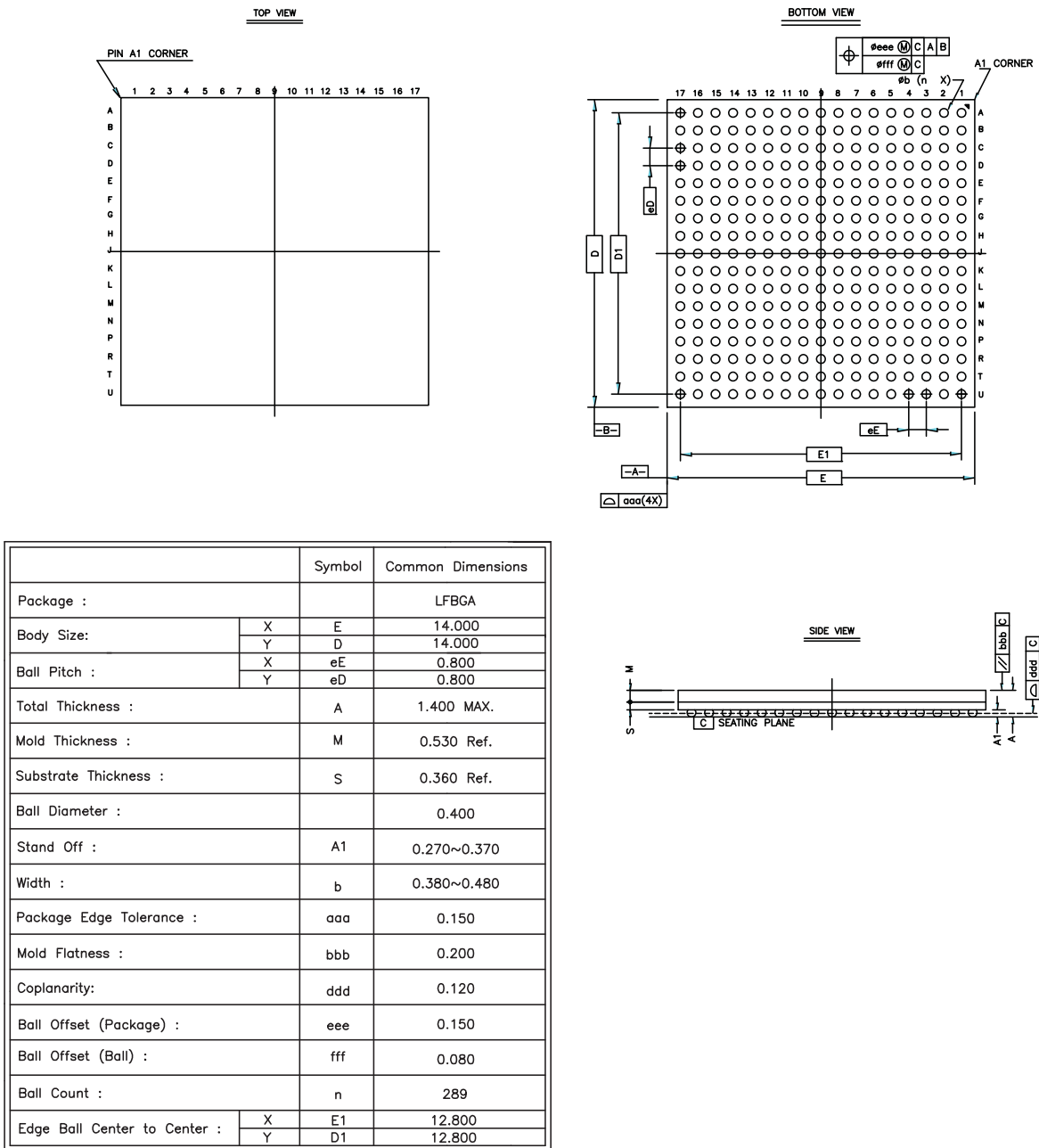
Figure 57-2. 289-ball LFBGA Package Drawing
