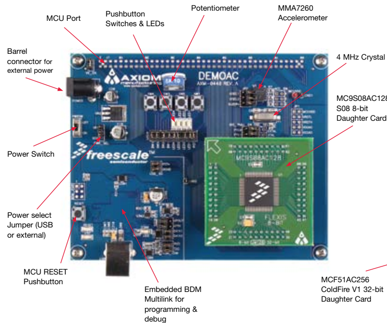
Figure 1. DEMOS08AC
