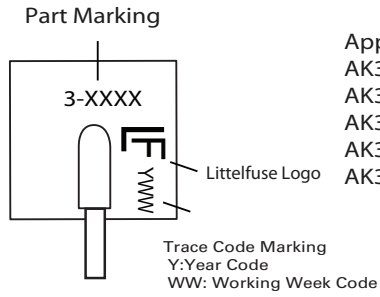
Type 1 - Side View
