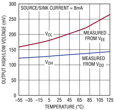
Output High/Low Voltage vs Temperature
