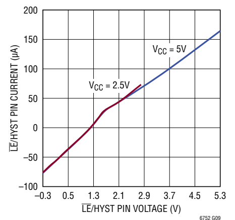
\overline{LE}/HYST Pin I-V Characteristics
