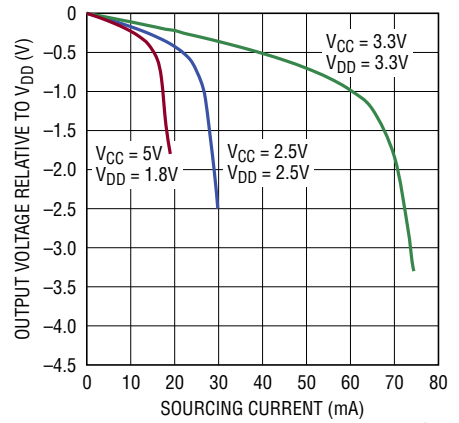
Output High Voltage vs Sourcing Current
