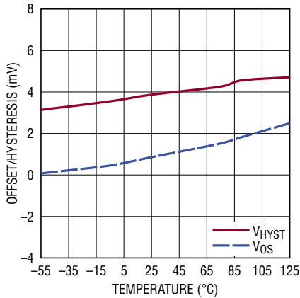
Input Offset Voltage and Hysteresis vs Temperature
