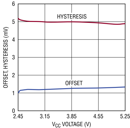
Input Offset Voltage and Hysteresis vs V_{CC} Voltage
