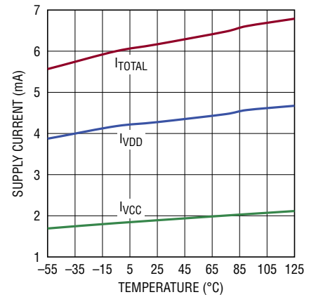
Supply Current vs Temperature (LTC6752-3)
