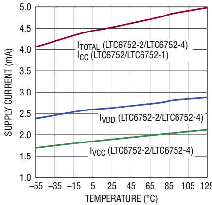
Supply Current vs Temperature (LTC6752/LTC6752-1/LTC6752-2/ LTC6752-4)
