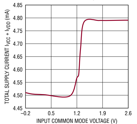
Supply Current vs Input Common Mode Voltage (LTC6752/LTC6752-1/ LTC6752-2/LTC6752-4)
