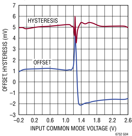
Input Offset Voltage and Hysteresis vs Input Common Mode
