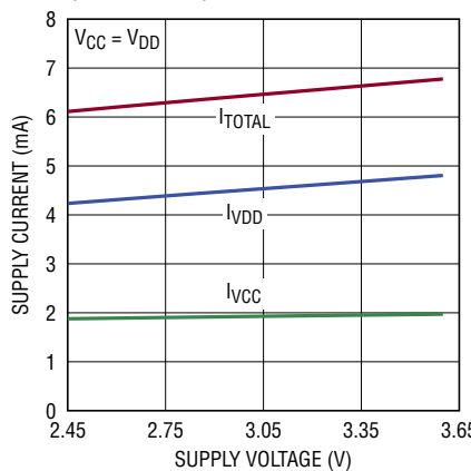
Supply Current vs Supply Voltage (LTC6752-3)
