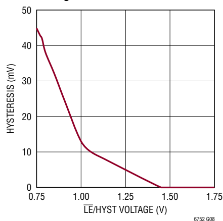
Input Hysteresis vs \overline{LE}/HYST Pin Voltage
