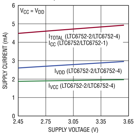
Supply Current vs Supply Voltage (LTC6752/LTC6752-1/LTC6752-2/ LTC6752-4)
