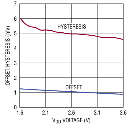
Input Offset Voltage and Hysteresis vs V_{DD} Voltage
