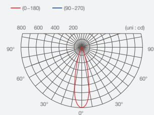
Light Distribution
