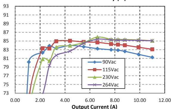
MVAD065-05 Efficiency (%)
