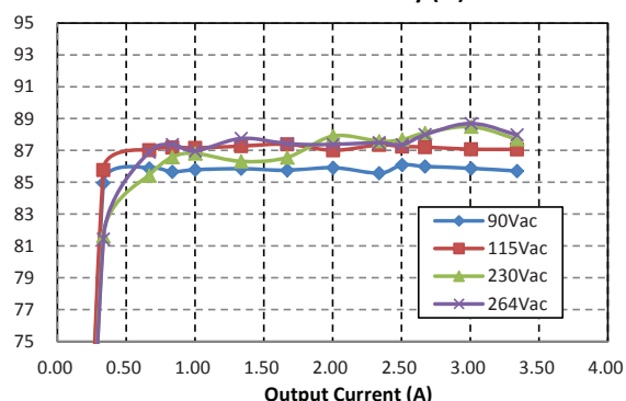
MVAD065-18 Efficiency (%)
