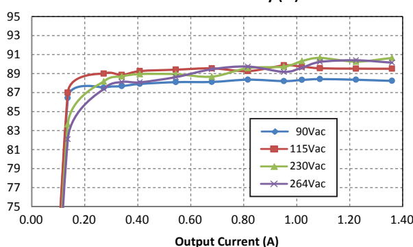
MVAD065-48 Efficiency (%)
