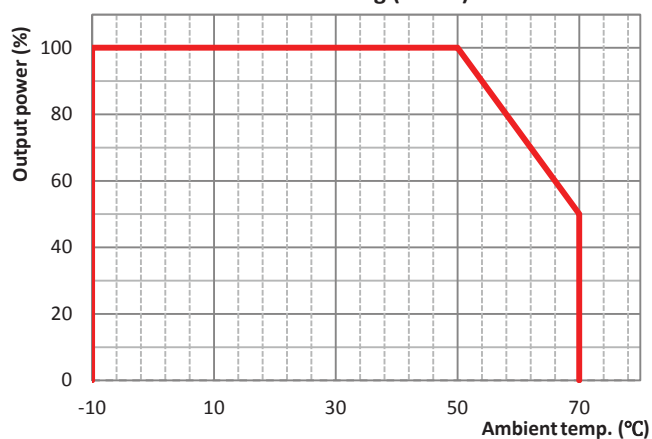
Thermal Derating (Other)
