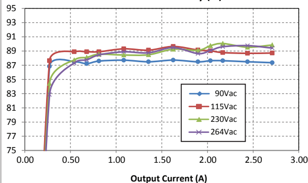
MVAD065-24 Efficiency (%)
