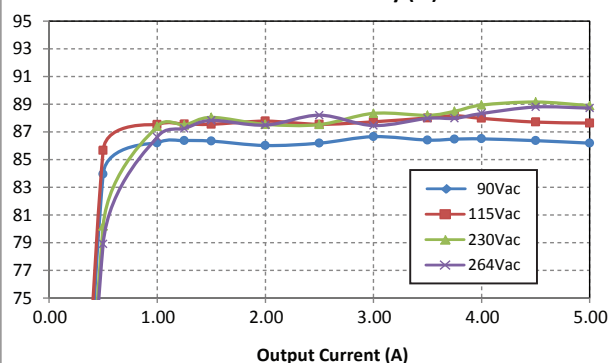
MVAD065-12 Efficiency (%)
