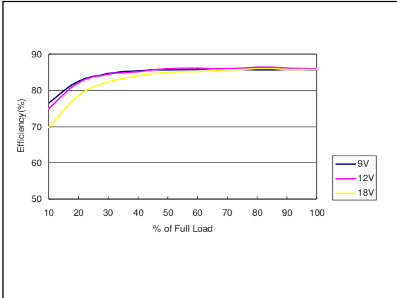
Figure 22: AEE00CC12-M Efficiency Versus Output Current Curve Vin = 9 to 18Vdc Load: Io = 0 to ±0.333
