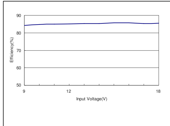
Figure 23: AEE00CC12-M Efficiency Versus Input Voltage Curve Vin = 9 to 18Vdc Load: Io = ±0.333
