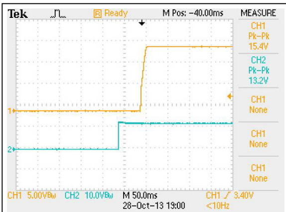
Figure 26: AEE00CC12-M Output Voltage Startup Characteristic by Vin Vin = 12Vdc Load: Io = ±0.333 Ch1: Vo1 Ch2: Vin
