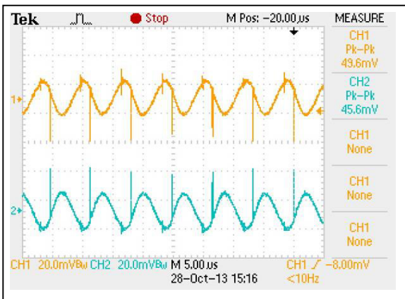
Figure 24: AEE00CC12-M Ripple and Noise Measurement Vin = 12Vdc Load: Io = ±0.333 Ch 1: Vo1 Ch 2: Vo2
