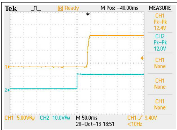
Figure 19: AEE00BB12-M Output Voltage Startup Characteristic by Vin Vin = 12Vdc Load: Io = ±0.417A Ch1: Vo1 Ch2: Vin
