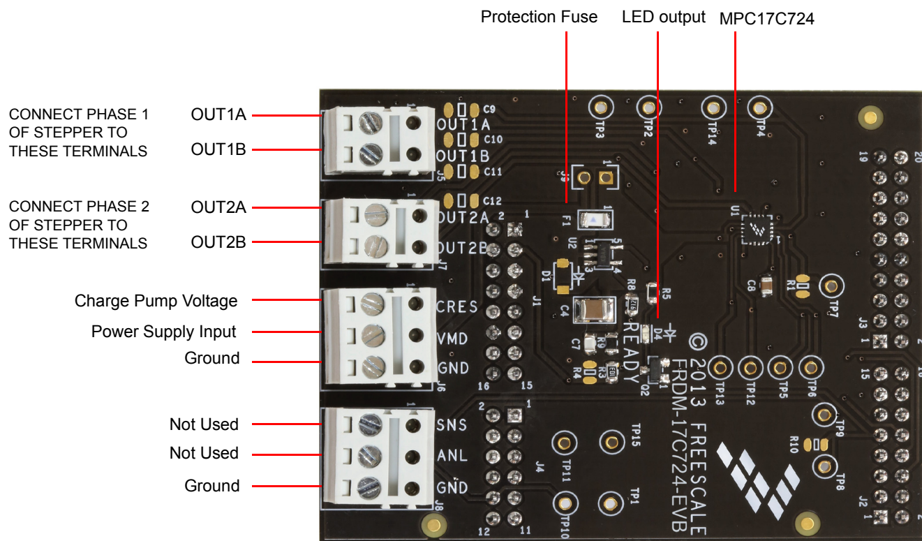
Figure 2. Board Description
