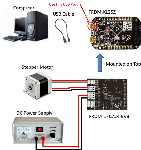
Figure 4. FRDM-17C724-EVB plus FRDM-KL25Z Board Setup
