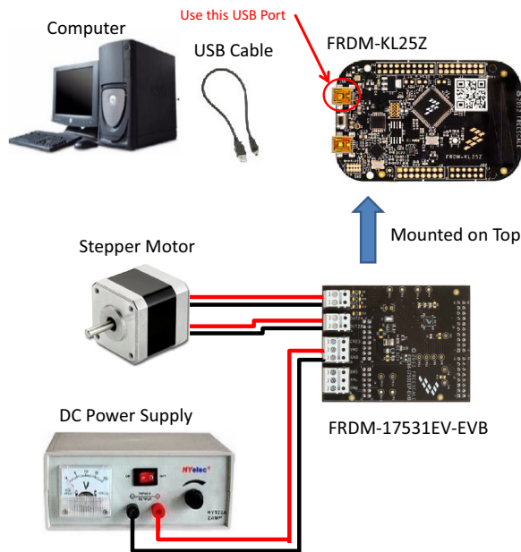
Figure 4. FRDM-17531EV-EVB plus FRDM-KL25Z Board Setup
