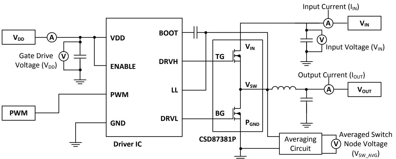
Figure 27. Typical Application
