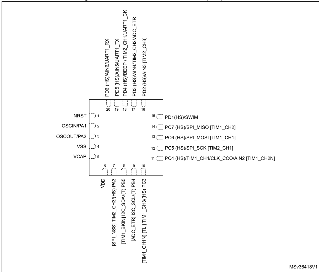
Figure 6. STM8S103Fx UFQFPN20-pin pinout
