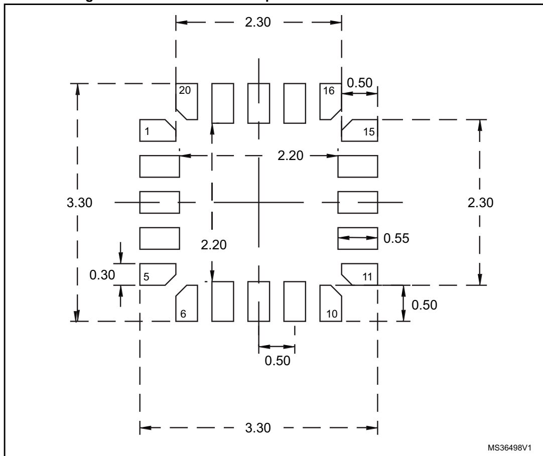
Figure 51. Recommended footprint without on-board emulation
