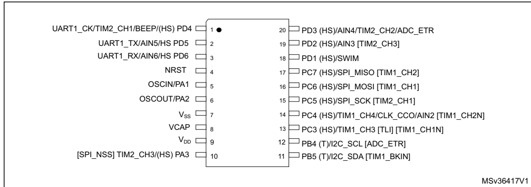
Figure 5. STM8S103Fx TSSOP20/SO20 pinout
