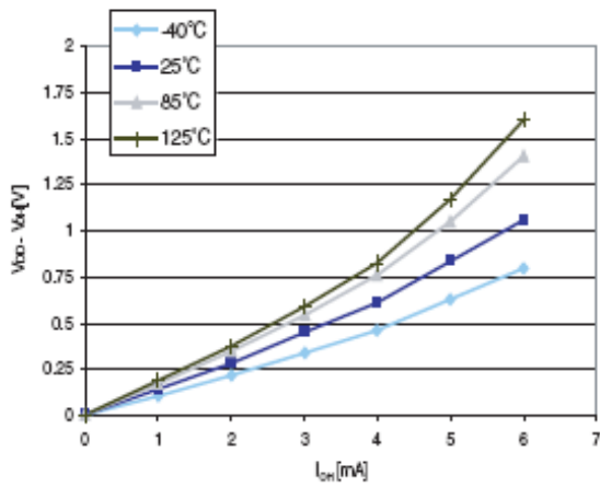
Figure 30. Typ. V_{DD} - V_{OH} @ V_{DD} = 3.3 V (standard ports)
