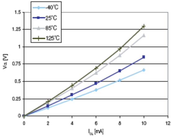
Figure 27. Typ. V_{OL} @ V_{DD} = 5.0 V (true open drain ports)
