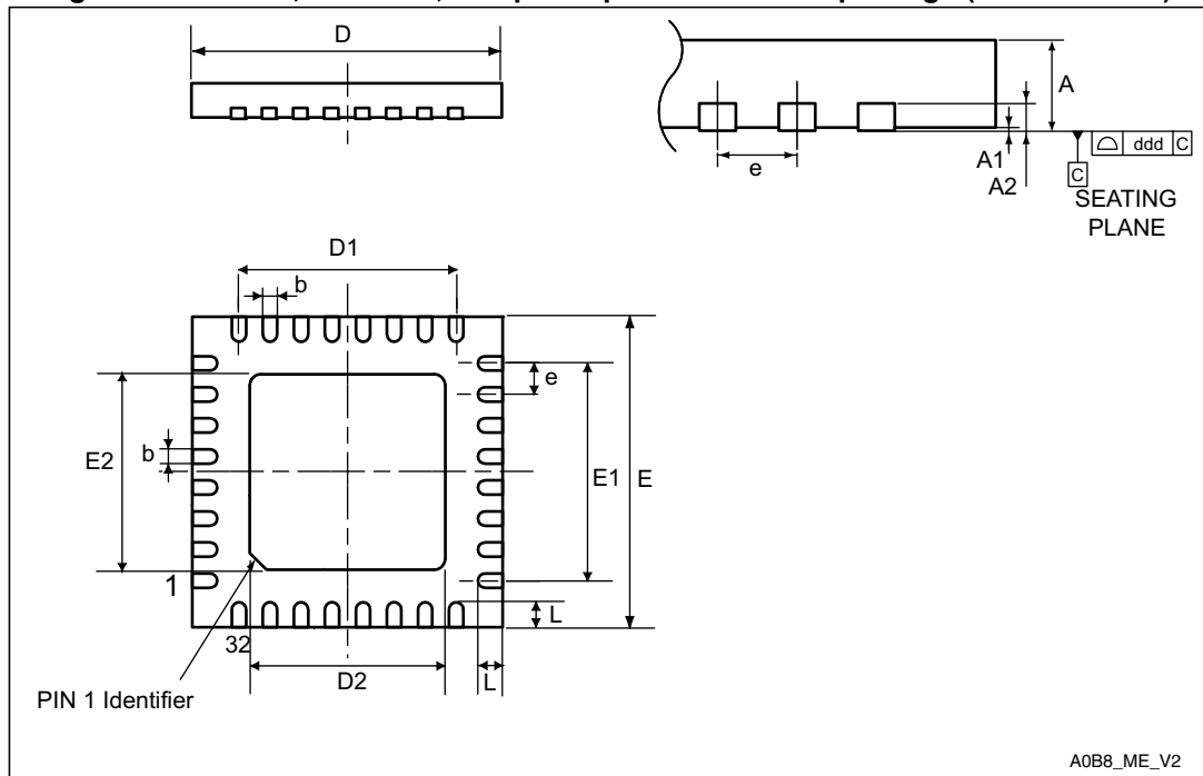
Figure 45. 32-lead, ultra thin, fine pitch quad flat no-lead package (5 mm x 5 mm)
