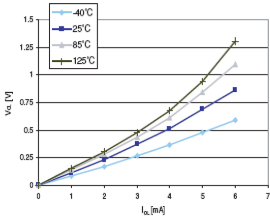
Figure 26. Typ. V_{OL} @ V_{DD} = 3.3 V (true open drain ports)
