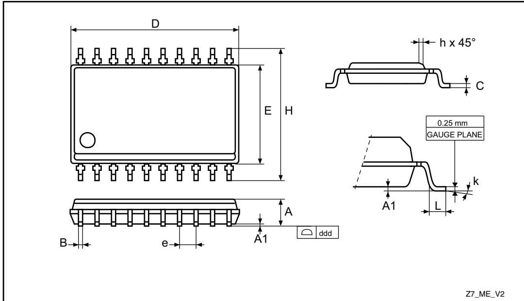
Figure 49. 20-lead, plastic small outline (300 mils) package
