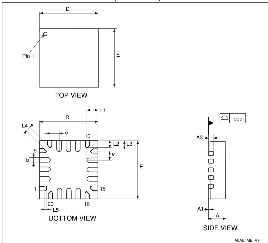
Figure 46. 20-lead, ultra thin, fine pitch quad flat no-lead package outline (3 mm x 3 mm)
