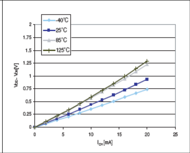
Figure 33. Typ. V_{DD} - V_{OH} @ V_{DD} = 5.0 V (high sink ports)
