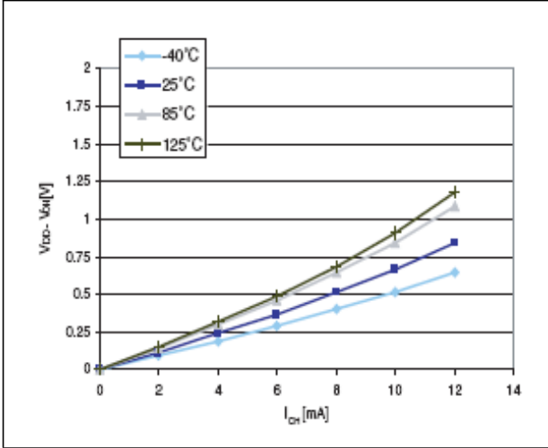
Figure 32. Typ. V_{DD} - V_{OH} @ V_{DD} = 3.3 V (high sink ports)
