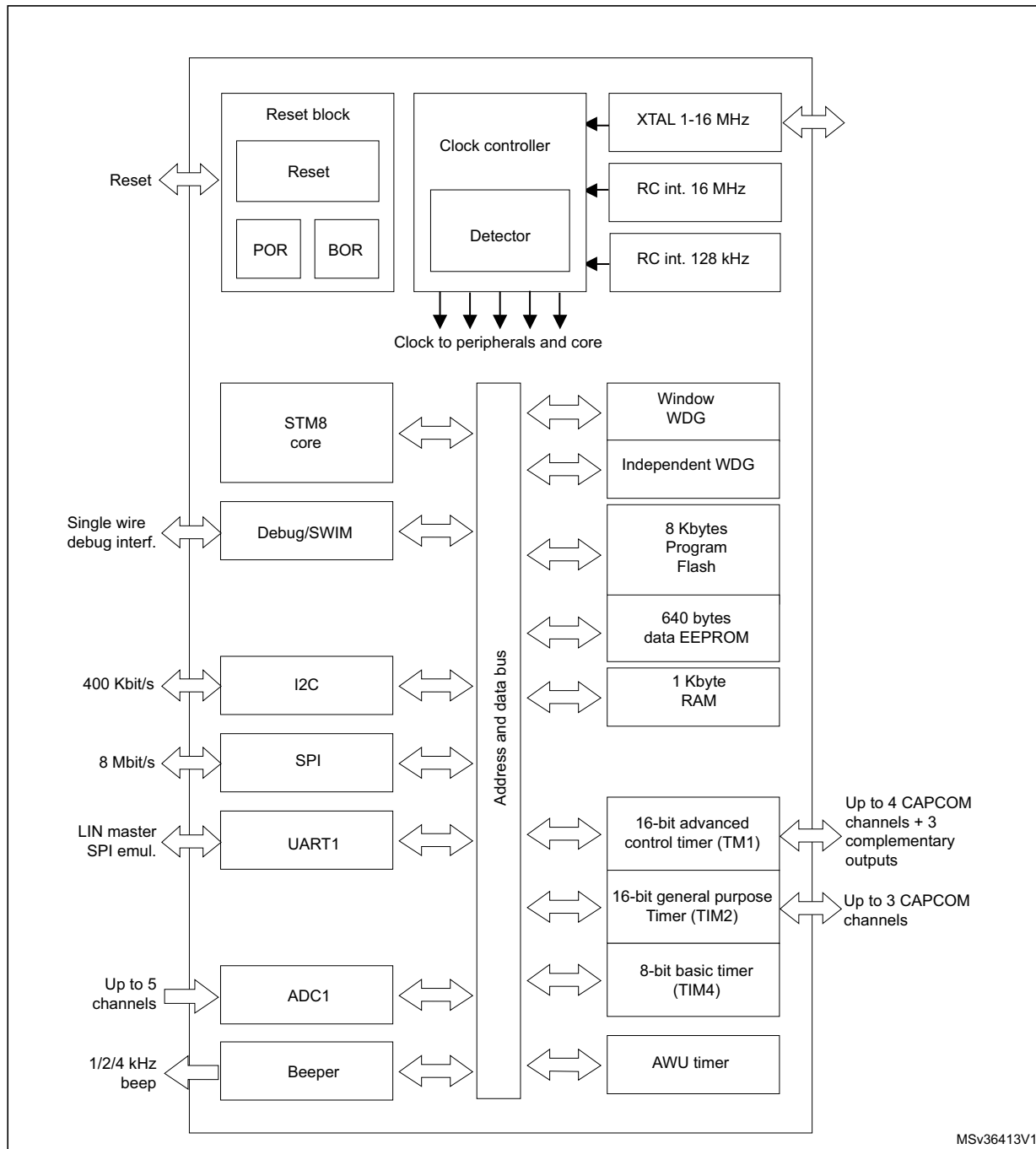
Figure 1. STM8S103x3/2 block diagram
