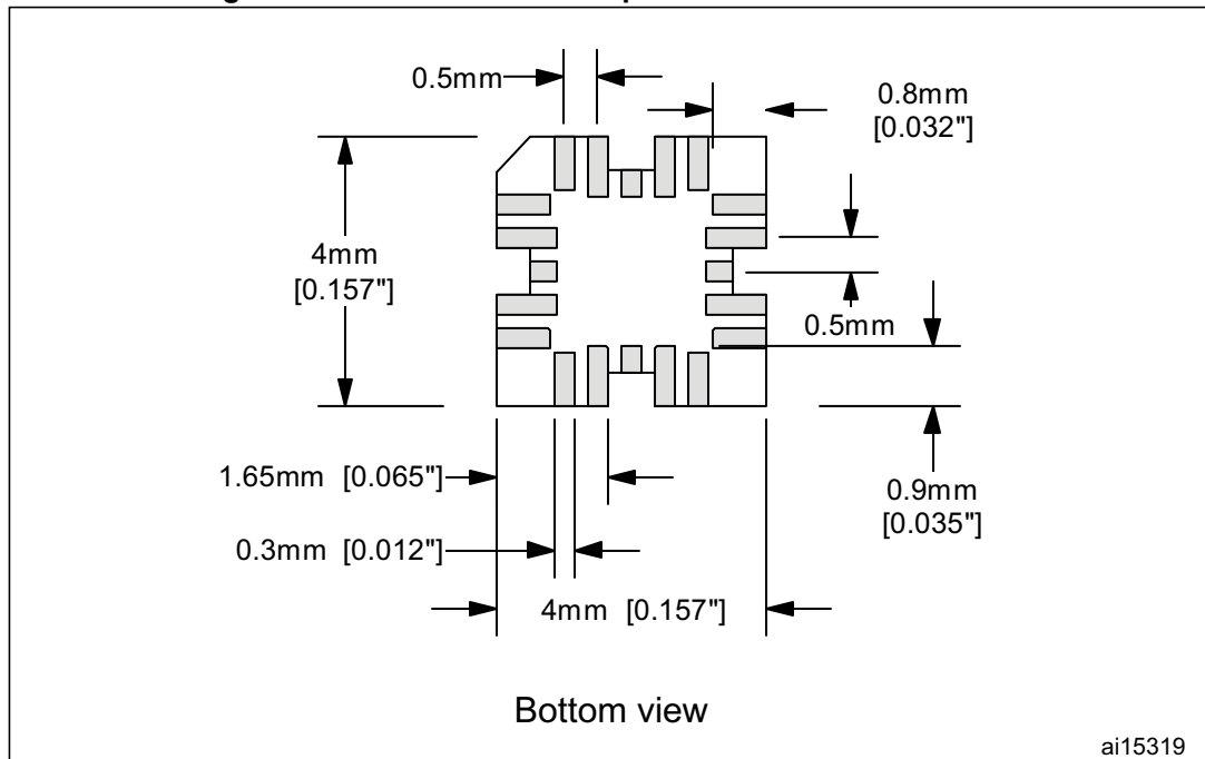
Figure 50. Recommended footprint for on-board emulation
