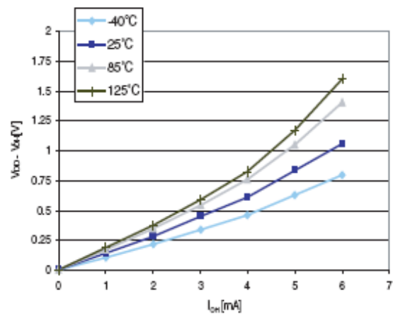
Figure 31. Typ. V_{DD} - V_{OH} @ V_{DD} = 5.0 V (standard ports)
