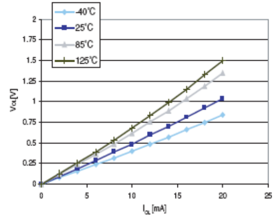
Figure 27. Typ. V_{OL} @ V_{DD} = 5.0 V (true open drain ports)
