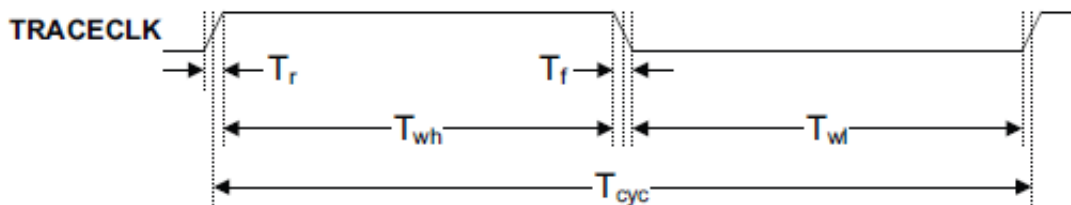
Figure 5. TRACE_CLKOUT specifications
