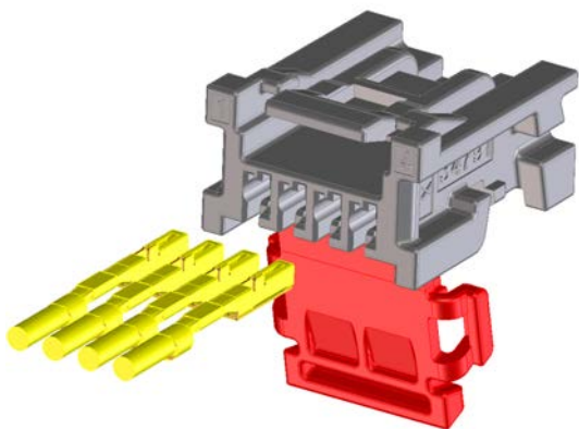
1. Insert Crimped Terminals
