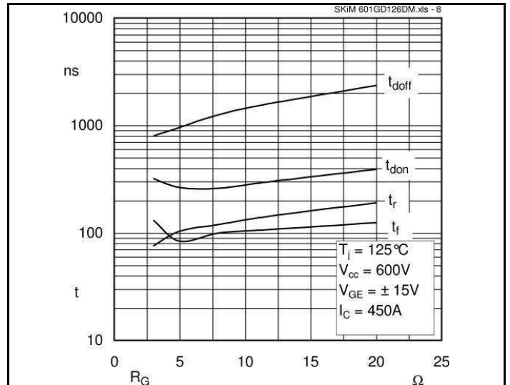
Fig. 8 Switching times vs. gate resistor R_G
