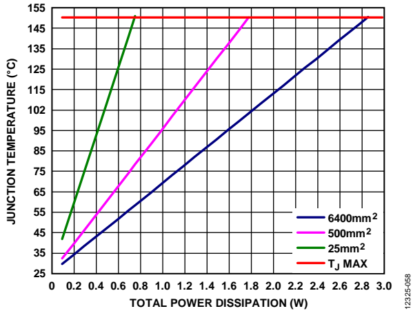
Figure 59. Junction Temperature vs. Total Power Dissipation for the 8-Lead SOIC, T_A = 25^\circ\text{C}
