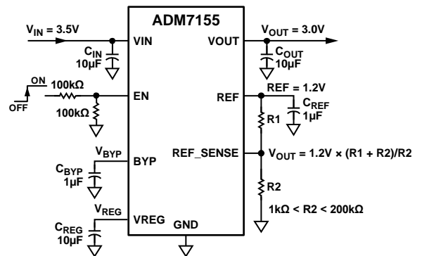
Figure 53. Typical EN Pin Voltage Divider
