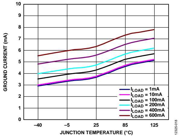
Figure 18. Ground Current vs. Junction Temperature ( T_J ) at Various Loads, V_{OUT} = 1.2\text{ V}
