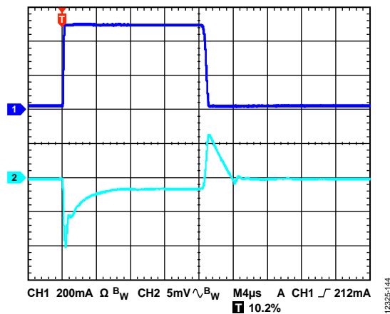
Figure 45. Output Transient Response, V_{\text{OUT}} = 3.3\text{ V} , C_{\text{OUT}} = 10\ \mu\text{F} , CH1 = Load Current, CH2 = V_{\text{OUT}}
