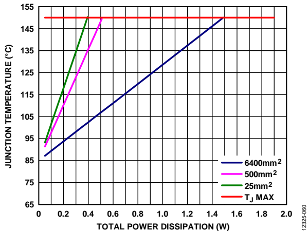
Figure 61. Junction Temperature vs. Total Power Dissipation for the 8-Lead SOIC, T_A = 85^\circ\text{C}
