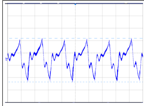
Figure 2: AVO200-48S05-6L Ripple and Noise Measurement Vin = 48Vdc Load: Io = 40A Ch 1: Vo (2us/div, 20mV/div)
