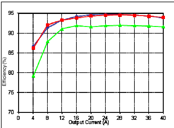
Figure 9: AVO200-48S05-6L Efficiency Curves @ 25 degC ◆ 36Vdc ◆ 48Vdc ▲ 75Vdc Loading: Io = 10% increment to 40A
