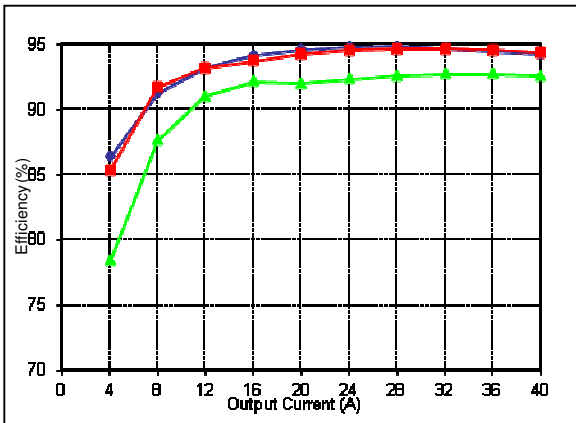
Figure 18: AVO200-48S05B-6L Efficiency Curves @ 25 degC Loading: Io = 10% increment to 40A
