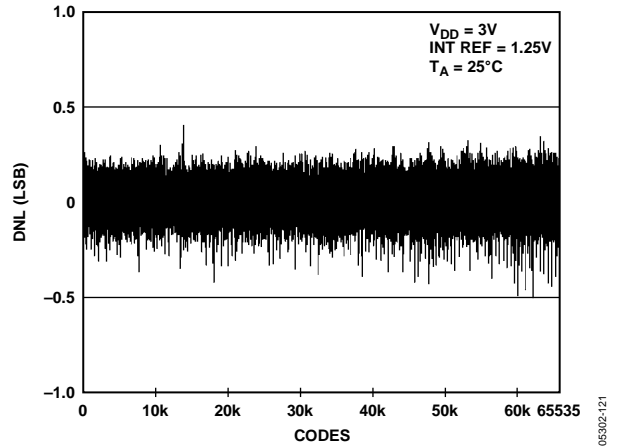
Figure 22. DNL AD5668-1
