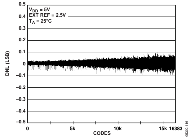
Figure 17. DNL AD5648-2
