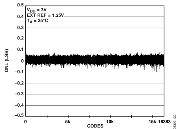
Figure 23. DNL AD5648-1
