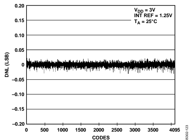
Figure 24. DNL AD5628-1
