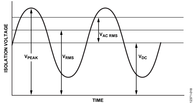
Figure 18. Critical Voltage Example
