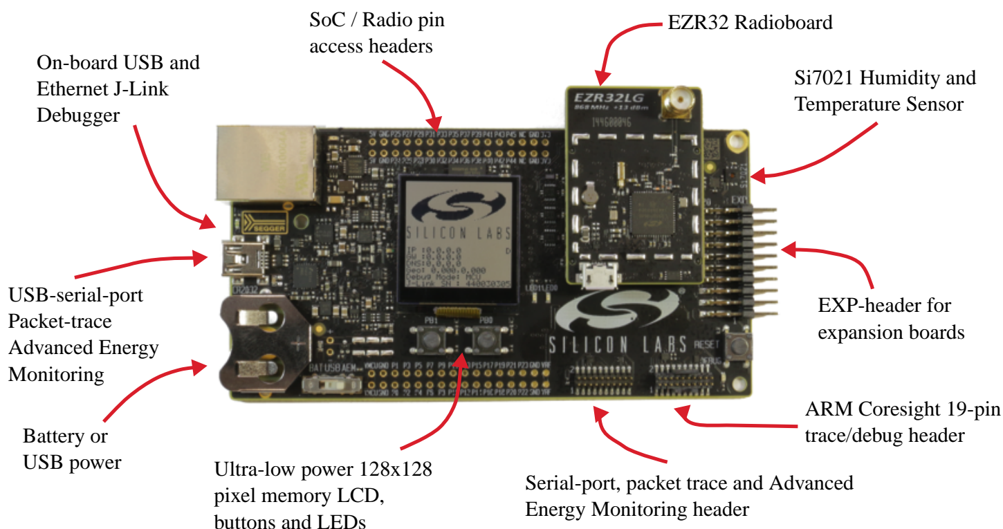
Figure 3.1. WSTK6201 hardware layout
