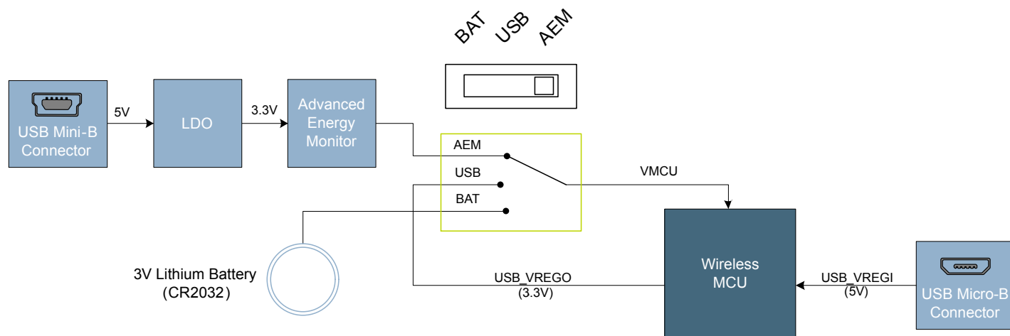
Figure 4.1. WSTK6201 Power Switch
