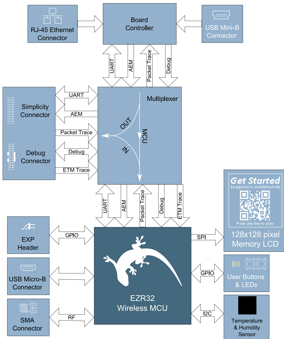
Figure 2.1. WSTK6201 Block Diagram
