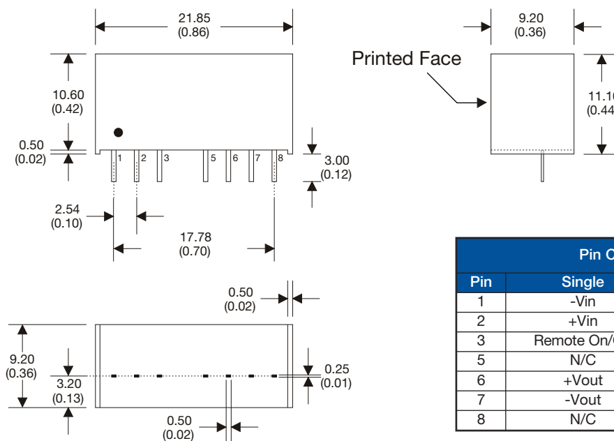
Pin Connections
