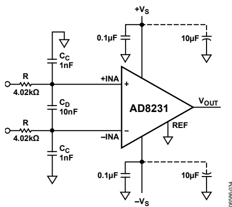
Figure 52. RFI Suppression
