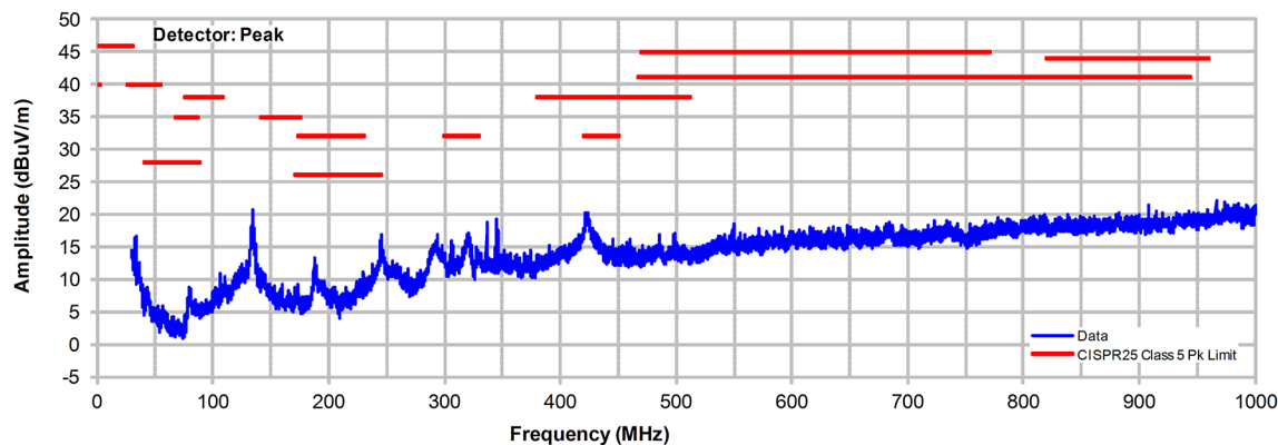
Figure 3. LT8609 Demo Circuit EMI Performance in CISPR25 Radiated Emission Test, Antenna Polarization: Horizontal ( V_{IN} = 14V , V_{OUT} = 5V , I_{OUT} = 2A , 2MHz Switching Frequency, Spread Spectrum Mode operation)
