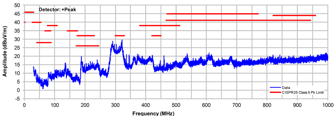
Figure 2. LT8609 Demo Circuit EMI Performance in CISPR25 Radiated Emission Test, Antenna Polarization: Vertical ( V_{IN} = 14V , V_{OUT} = 5V , I_{OUT} = 2A , 2MHz Switching Frequency, Spread Spectrum Mode operation)
