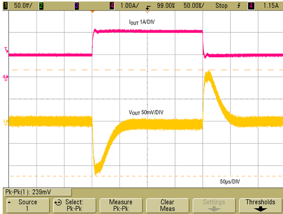
Figure 6. DC2195A 1A to 2A Load Transient
