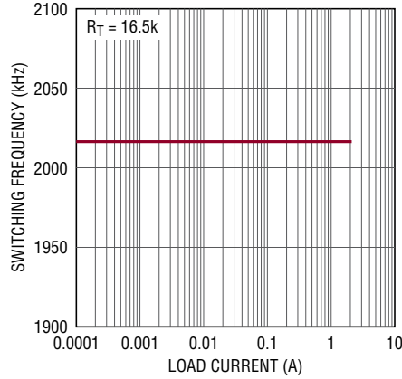
Switching Frequency vs I_{\text{LOAD}}
