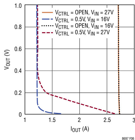
Figure 6. Output Current Regulation vs V_{OUT} at f_{SW} = 2\text{MHz} , R_{SENSE} = 18\text{m}\Omega
