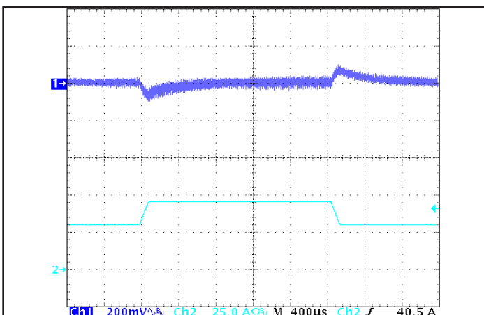
Figure 5: Output voltage response to step-change in load current (50% -75% -50% of I_{out(max)} ; dI/dt = 0.2 A/\mu s ). Load cap: 15 \mu F tantalum and 1 \mu F ceramic capacitors. Ch 1: V_{out} , Ch 2: I_{out} .
