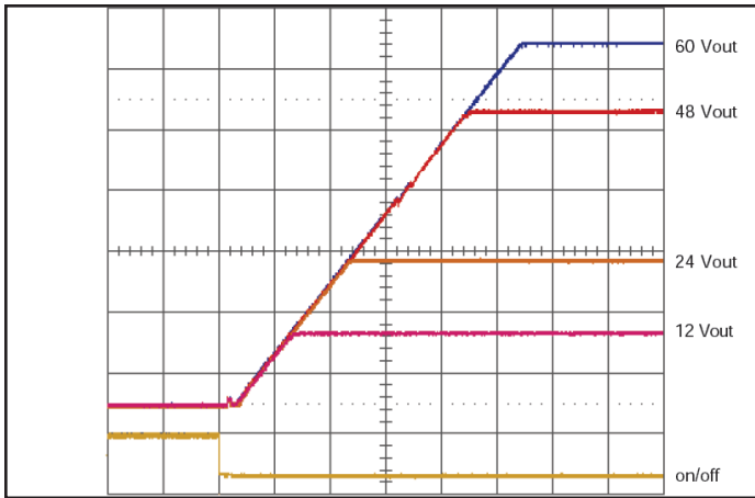
Figure 7: Turn-on transient at 36V input; full load (20ms/div). ON/OFF input (5V/div) Ch 1-4: Vout (10V/div)
