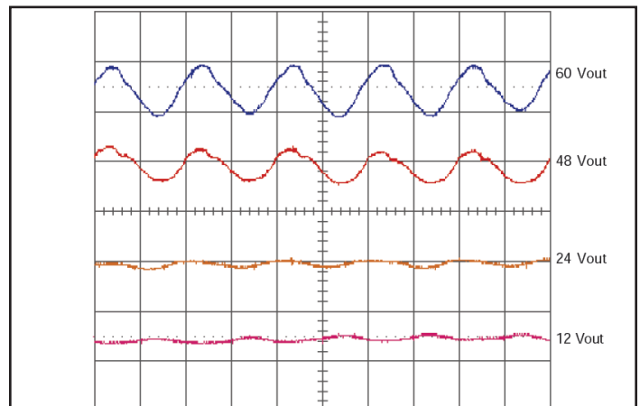
Figure 6: Output Voltage Ripple at 36V input and rated load current (50mV/div). Load capacitance: 100µF electrolytic cap.. Bandwidth: 20MHz. See Figure 4.
