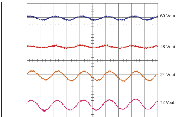
Figure 5: Input Terminal Ripple Current at 36V input and rated load current (500mA/div). Load capacitance: 100µF electrolytic cap. Bandwidth: 20MHz. See Figure 4
