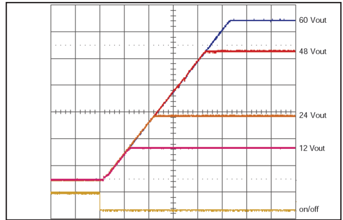
Figure 8: Turn-on transient at 36V input; zero load (20ms/div). ON/OFF input (5V/div) Ch 1-4: Vout (10V/div)
