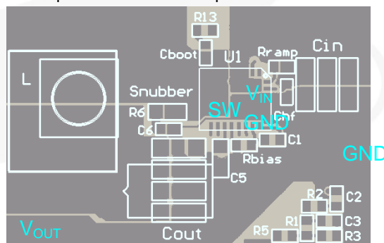
Figure 35. Recommended PCB Layout
