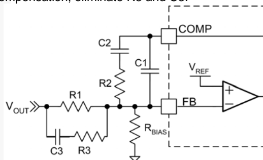
Figure 34. Compensation Network
