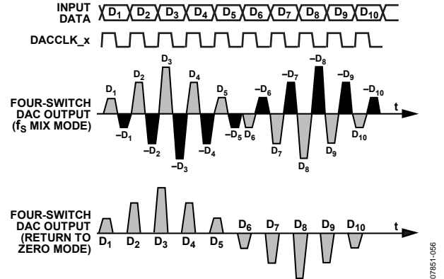
Figure 56. Mix-Mode and RZ DAC Waveforms
