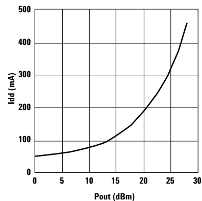
Figure 11. Idd vs. Pout.
