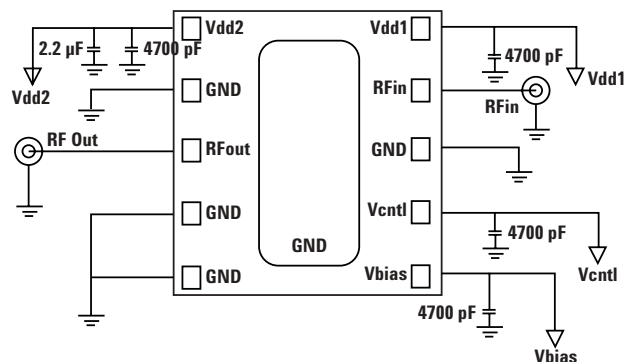
Figure 20. ACPM-7833 Evaluation Board Schematic and Layout.
