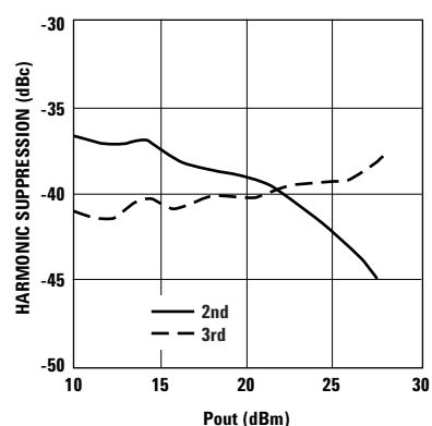
Figure 14. Harmonic Suppression vs. Pout.
