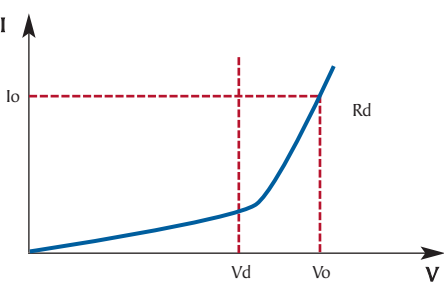
LED I-V Curve
