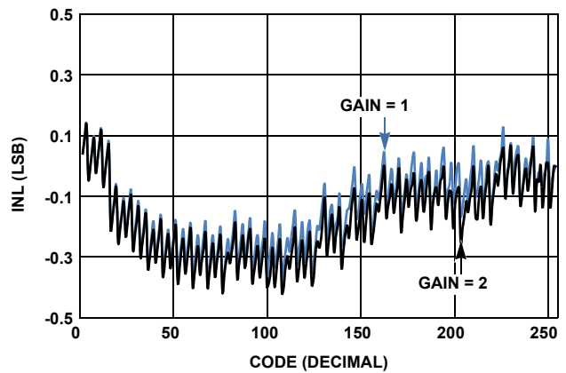
FIGURE 11. GP DAC INL vs CODE V_{DD} = 15V
