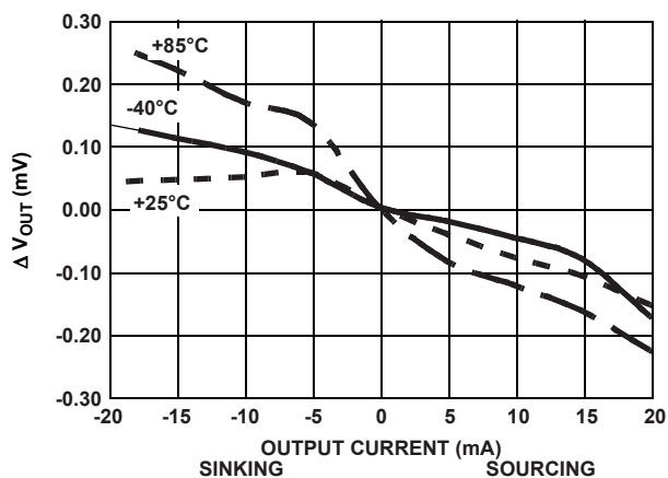
FIGURE 11. LOAD REGULATION
