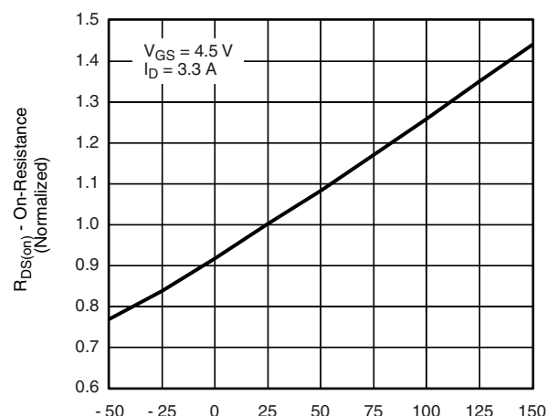
T_J - Junction Temperature (°C) On-Resistance vs. Junction Temperature
