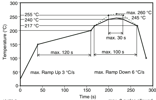
Fig. 6 - Vishay Lead (Pb)-free Reflow Soldering Profile (acc. to J-STD-020C)
