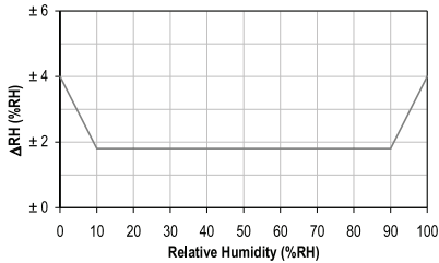
Figure I.1 RH Accuracy Chart
