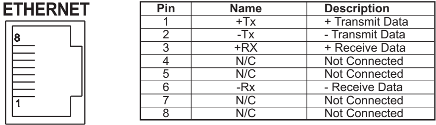
Figure 2.10 RJ45 Pinout
