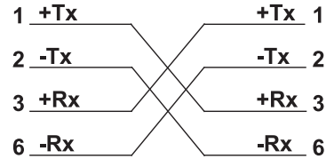
Figure 2.11 10BASE-T Crossover Cable Wiring
