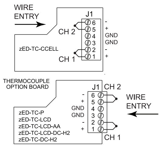
Figure 2.12 Thermocouple Wiring and TC Wire Color Chart
