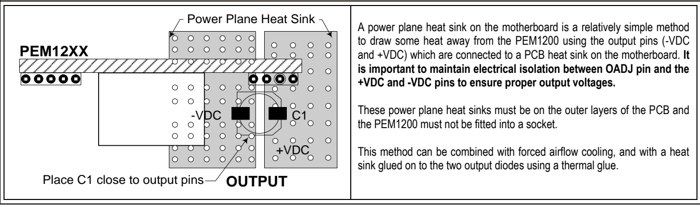
Figure 8 – Power Plane Heat Sink
