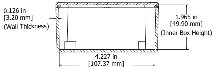
SECTION L-L Side View of Assembly
