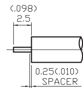
STRIPPING DIMENSION
