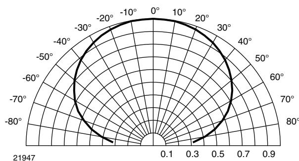
Fig. 8 - Horizontal Directivity
