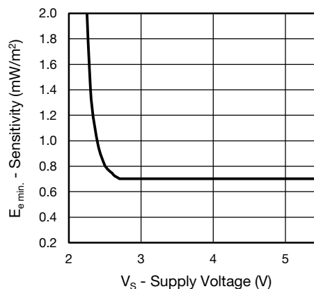
Fig. 7 - Sensitivity vs. Supply Voltage
