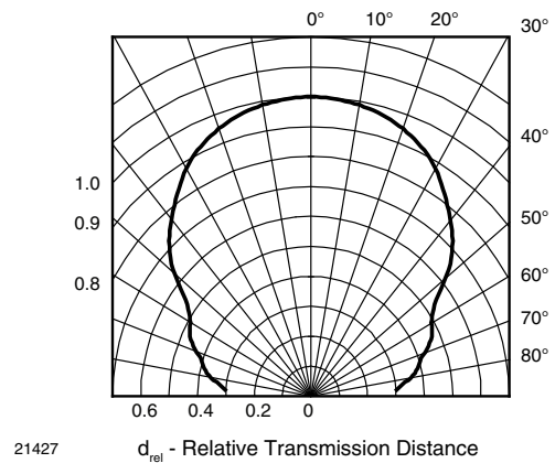
Fig. 8 - Horizontal Directivity
