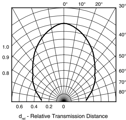
d_{rel} - Relative Transmission Distance
