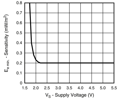
Fig. 10 - Sensitivity vs. Supply Voltage
