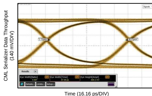
Figure 16. TL = 10 Inch 4-Mil FR4 Trace, DS100BR111A CHA, 10.3125 Gbps
