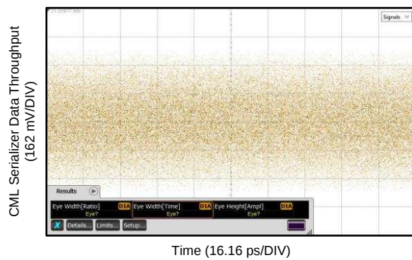
Figure 31. TL1 = 15 Inch 4-Mil FR4 Trace, TL2 = 10 Inch 4-Mil FR4 Trace, No Repeater, 10.3125 Gbps
