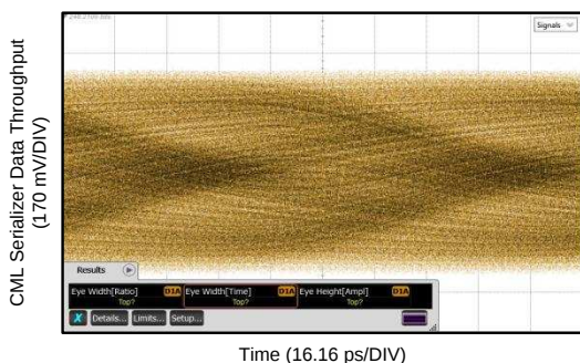
Figure 17. TL = 15 Inch 4-Mil FR4 Trace, No Repeater, 10.3125 Gbps
