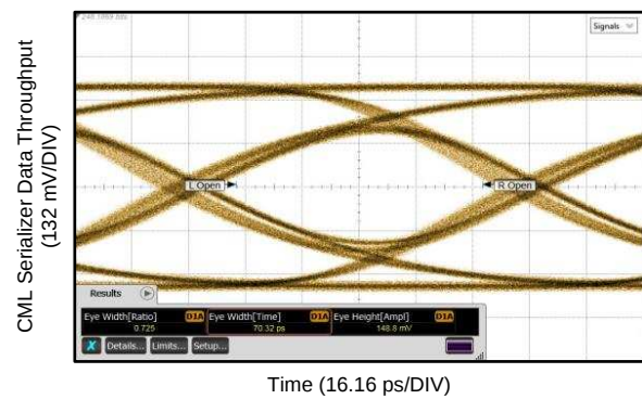
Figure 32. TL1 = 15 Inch 4-Mil FR4 Trace, TL2 = 10 Inch 4-Mil FR4 Trace, DS100BR111A CHA, 10.3125 Gbps
