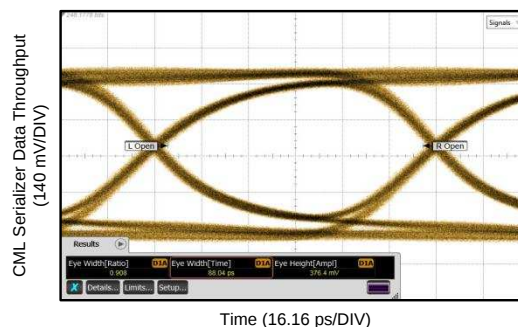
Figure 14. TL = 5 Inch 4-Mil FR4 Trace, DS100BR111A CHA, 10.3125 Gbps
