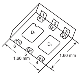
PowerPAK SC75-6L-Dual
