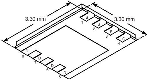
PowerPAK® 1212-8
