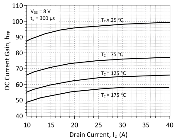
Figure 6: DC Current Gain vs. Drain Current
