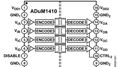
Figure 1. ADuM1410
