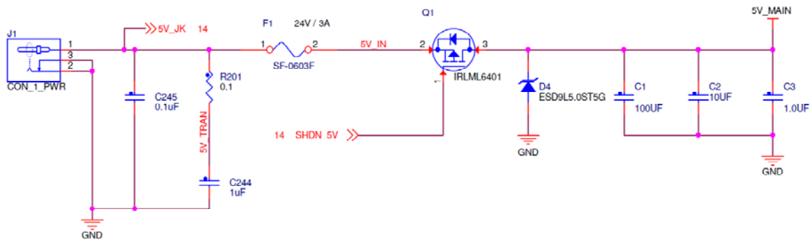
Figure 15. Board Main Power Circuit.
