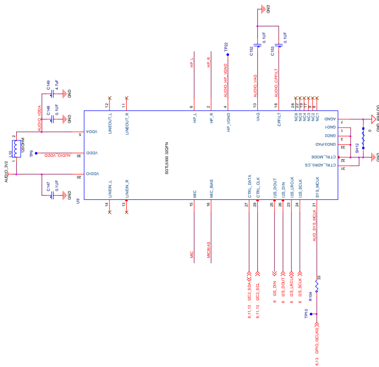
Figure 50. MX53 AUDIO
